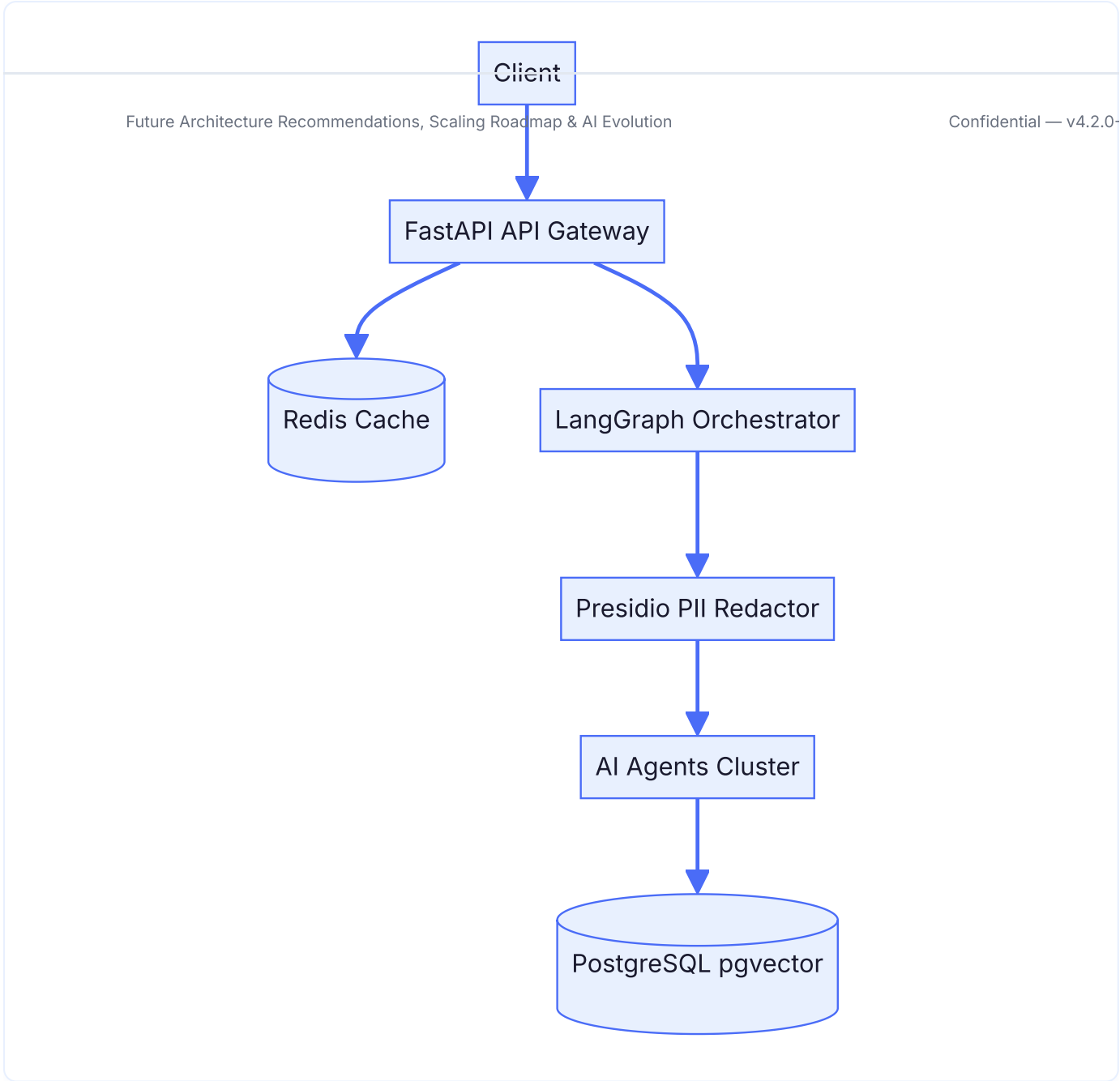
Figure 3.1: High-Level Proposed Nimblize Architecture. This diagram details the top-to-bottom layout of the system, showing the placement of security middleware, caches, orchestrators, and databases.
