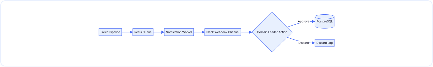
Figure 11.1: Proposed HITL Review Architecture. This diagram details the path of a flagged low-confidence payload, showing routing from Redis queues to Slack alert networks for manual resolution.
