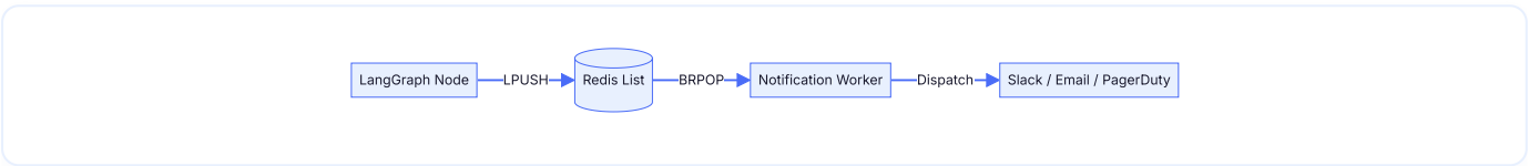
Figure 11.2: Proposed Redis Queue Workflow. This diagram illustrates the asynchronous dispatch flow utilizing Redis LPUSH/BRPOP operations.
