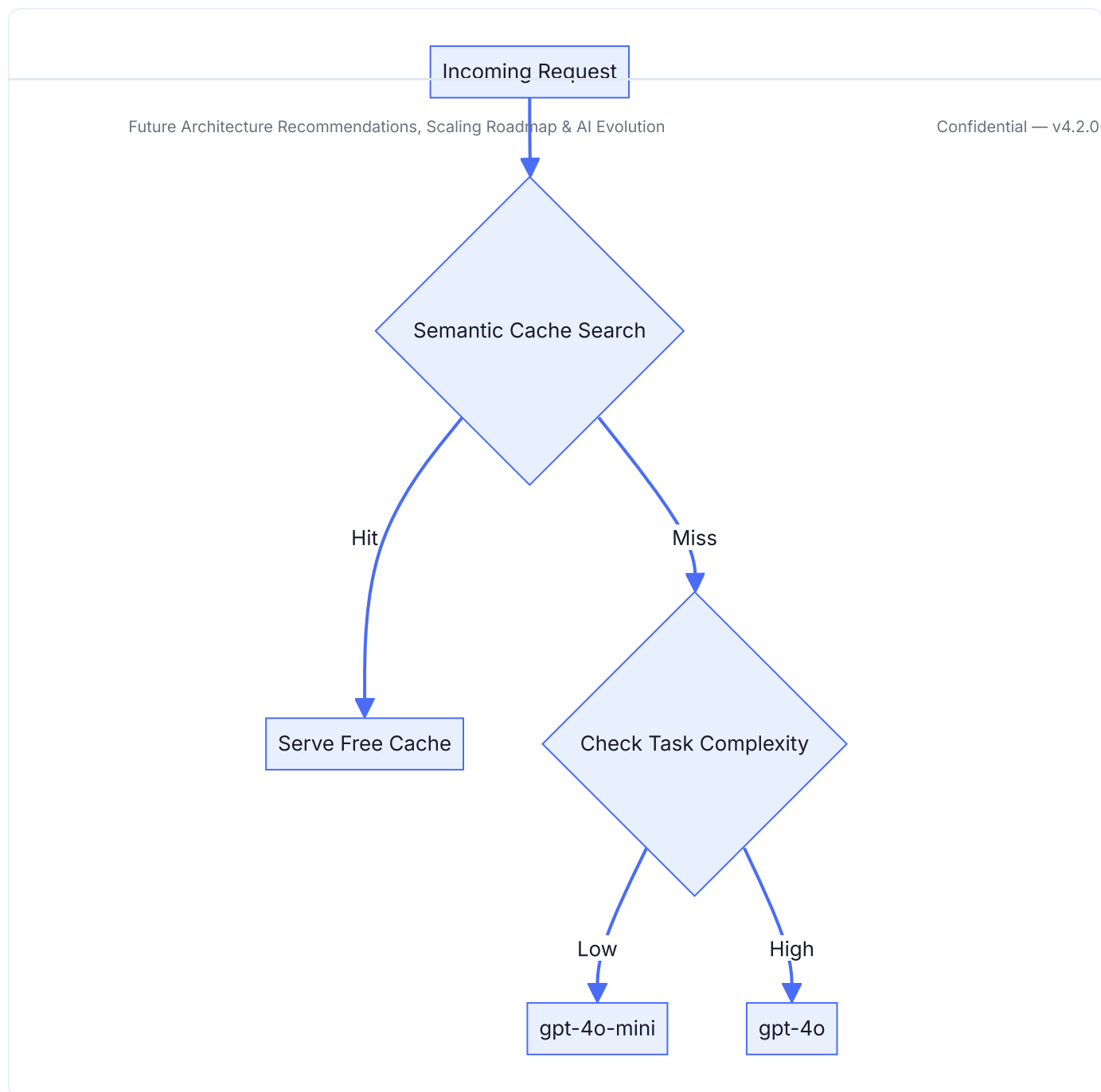
Figure 12.1: Proposed Cost Optimization Flow. This flowchart shows how incoming requests are filtered to minimize token costs, either via cache retrieval or tiered routing.
