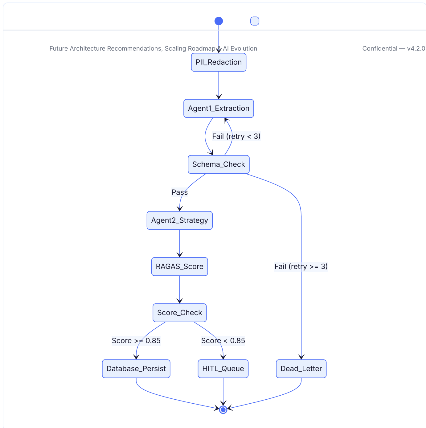
Figure 6.1: Proposed LangGraph State Machine. This state machine charts all conditional path choices from PII redaction to database commit, dead-letter storage, or HITL queue routing.
