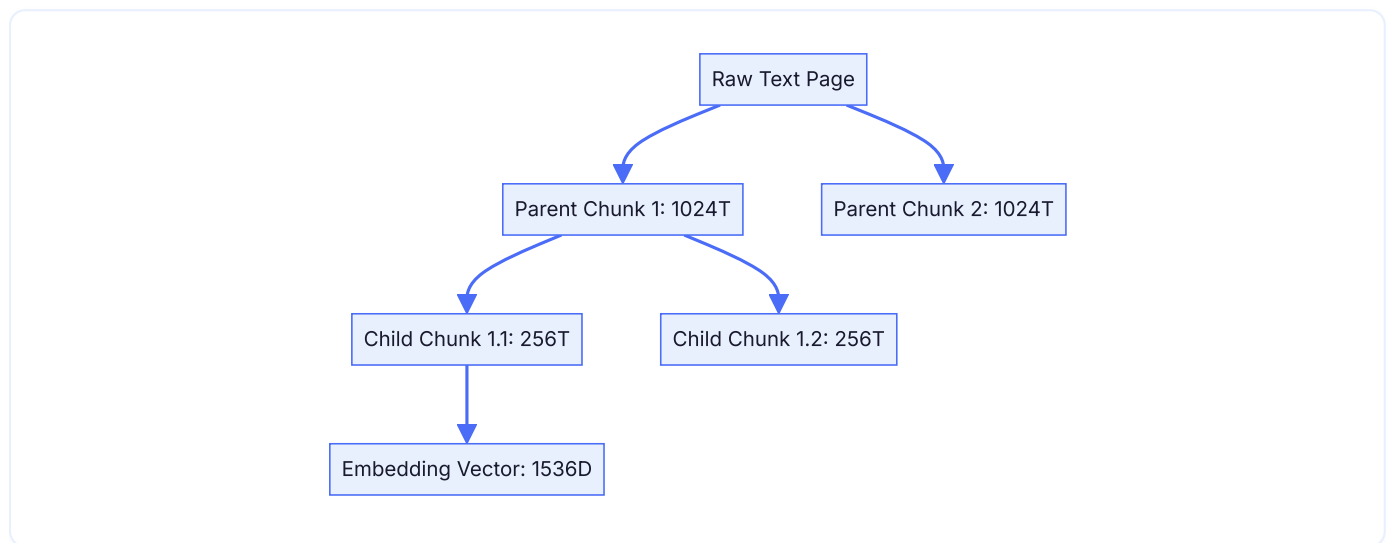
Figure 7.1: Parent-Child Chunking Layout. This diagram shows the relationship between parent chunks used for synthesis and child chunks embedded for vector similarity matching.
