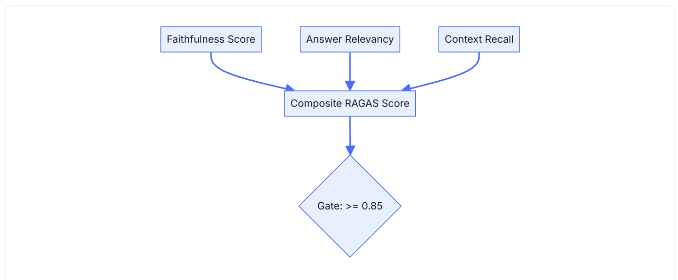
Figure 10.1: Proposed RAGAS Evaluation Pipeline. This diagram shows the three metrics combined into a single composite score to gate database writes.
