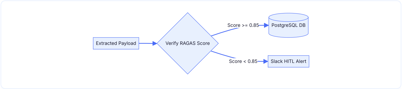
Figure 9.1: Proposed Confidence Gate Workflow. This diagram highlights how extracted payloads are routed depending on the composite RAGAS confidence score.
