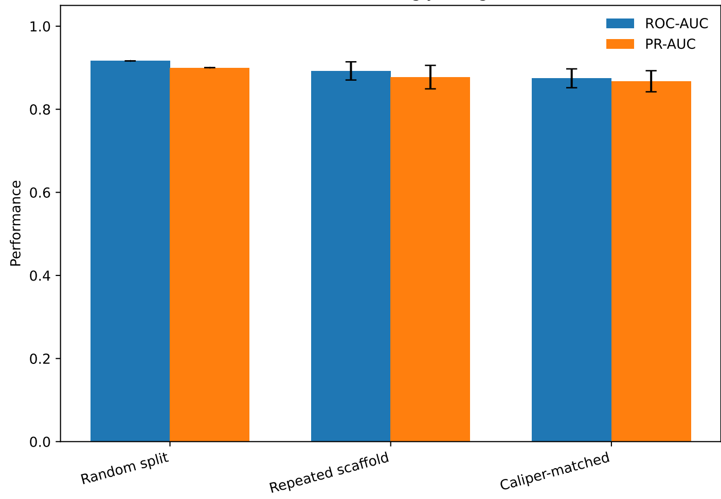
Performance under increasingly stringent evaluation
