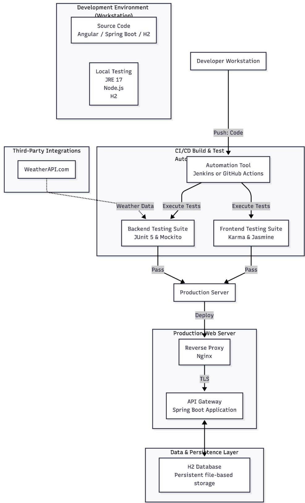
Figure 6 — Deployment Diagram
