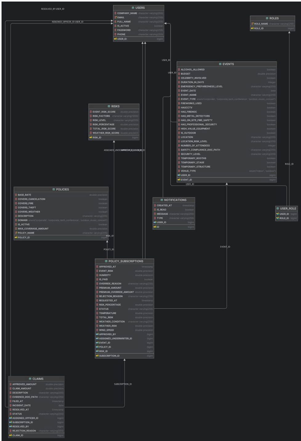
Figure 1 — Event Rakshak Entity Relationship Diagram (Full Data Model with Foreign Keys and Cardinalities)
