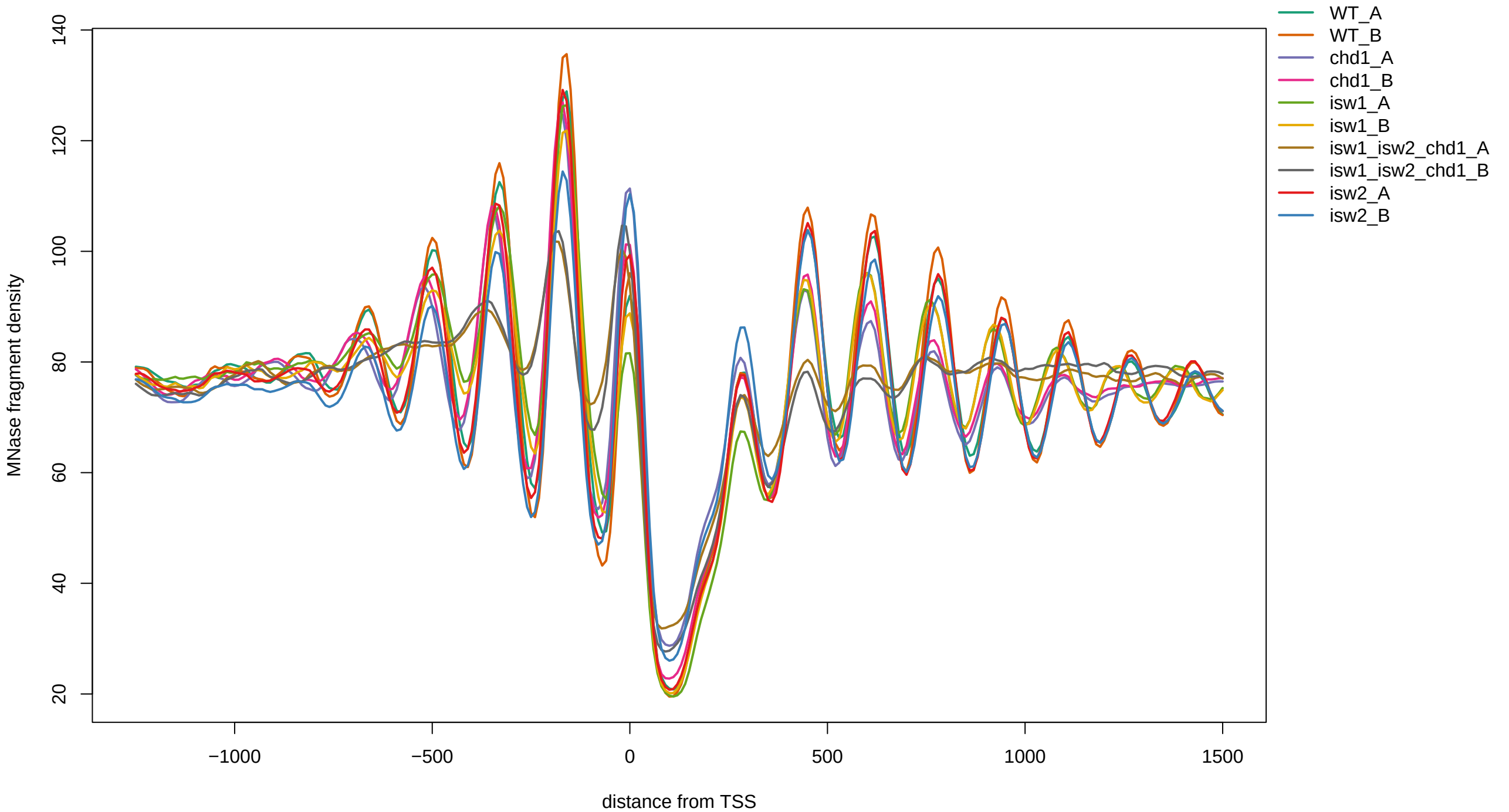
TSS profile: all samples (./tss_out_individual_plot/tss_out_individual_plot)
