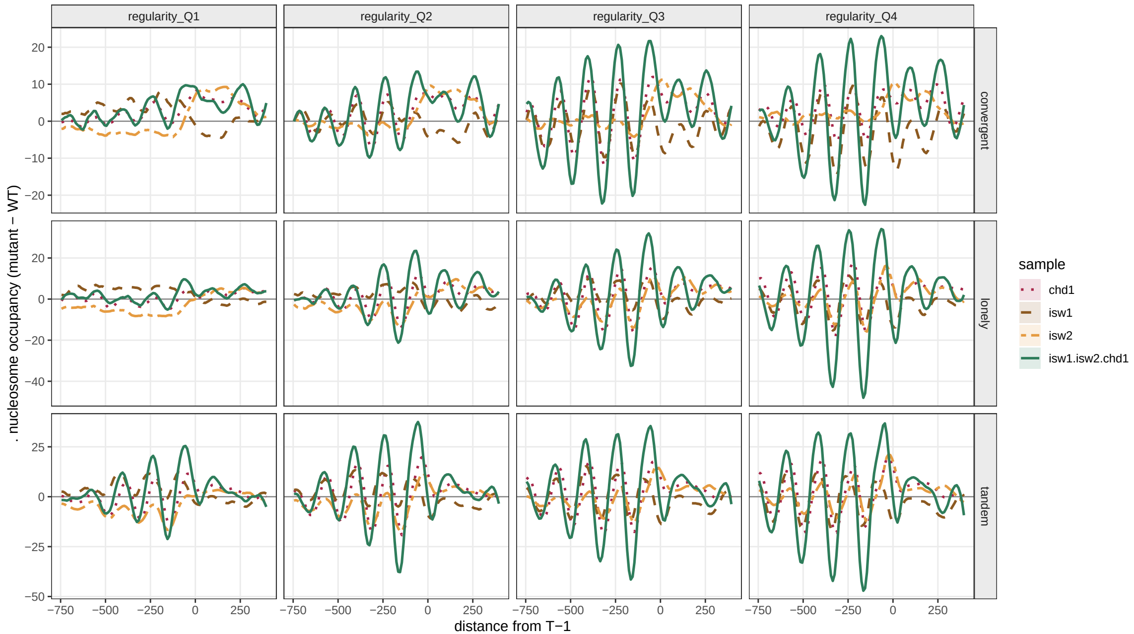
Normalized nucleosome occupancy: mutant – WT
