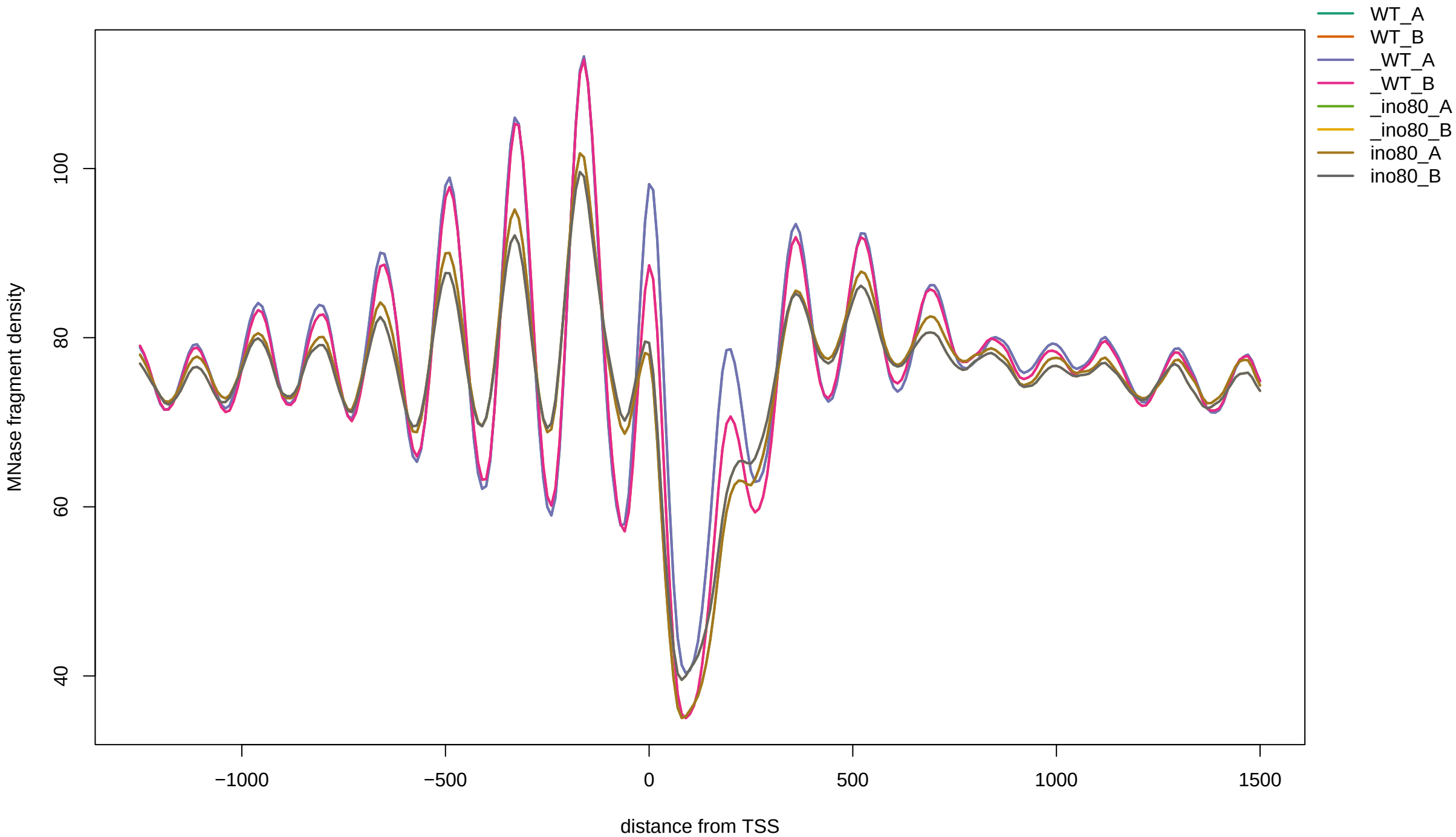
TSS profile: all samples (./TES_convergent_out_individual_plot/TES_convergent_out_individual_plot)
