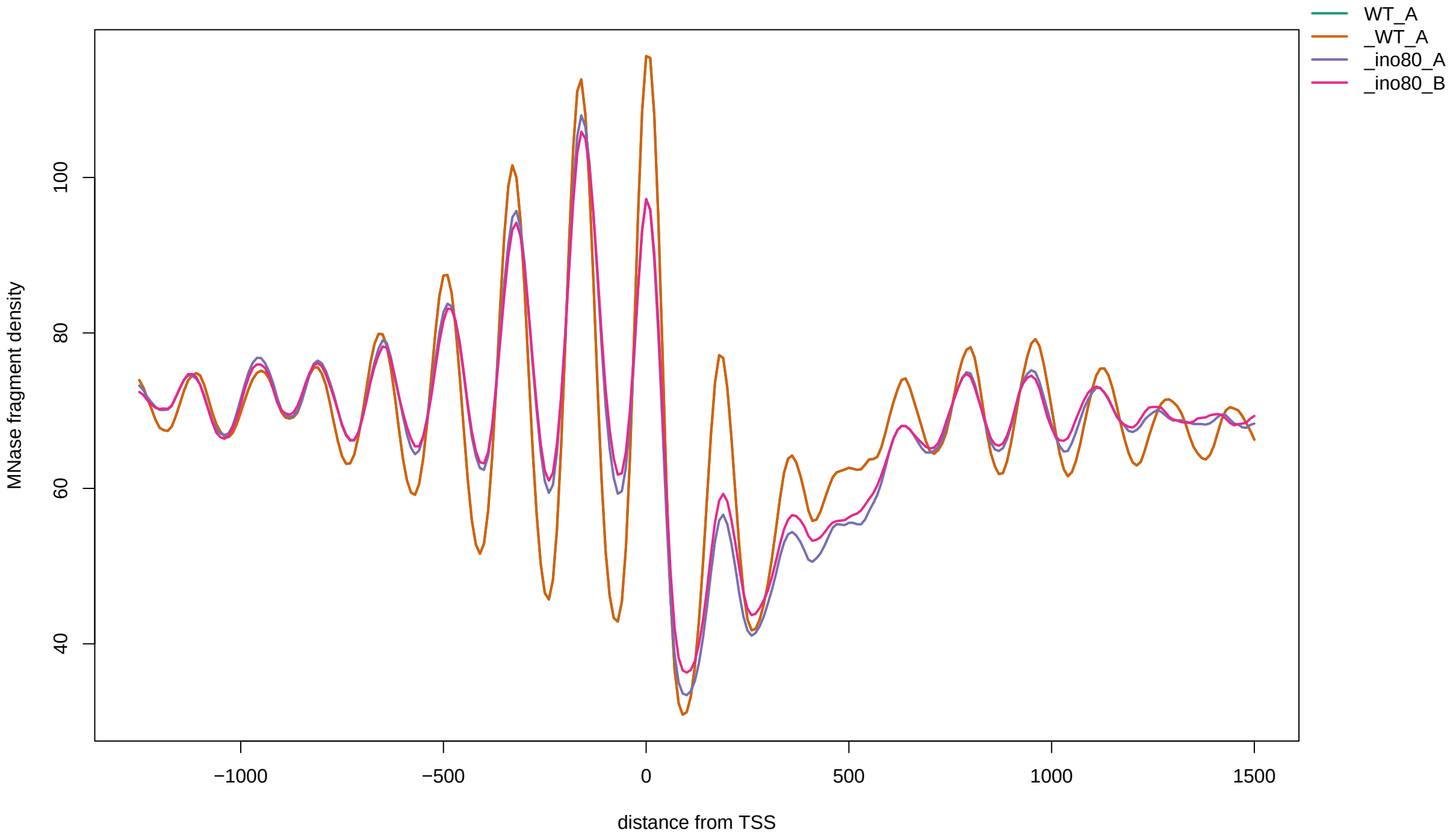
TSS profile: _ino80 vs WT_A
