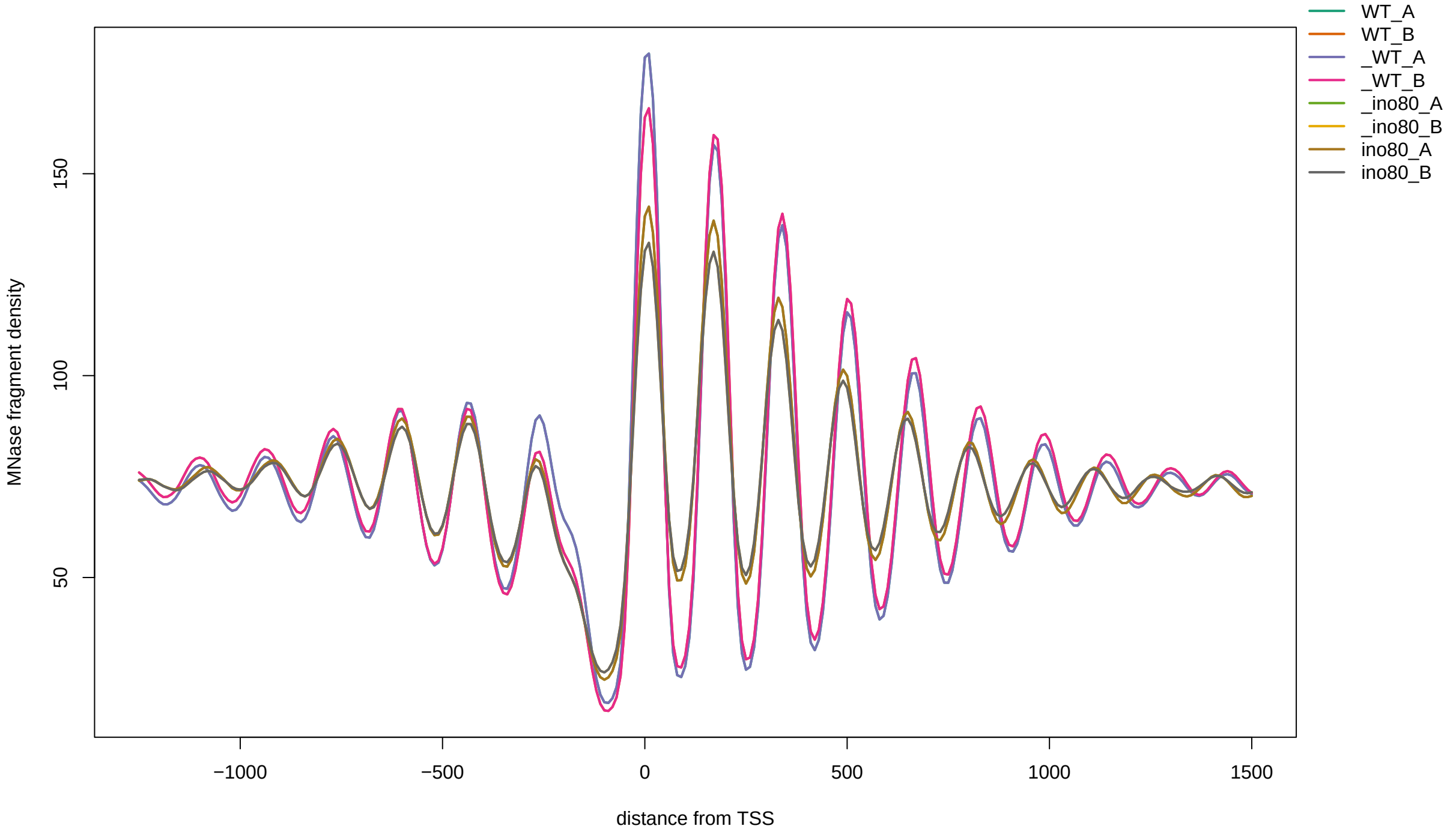
TSS profile: all samples (./plus1_out_plot/plus1_out_plot)
