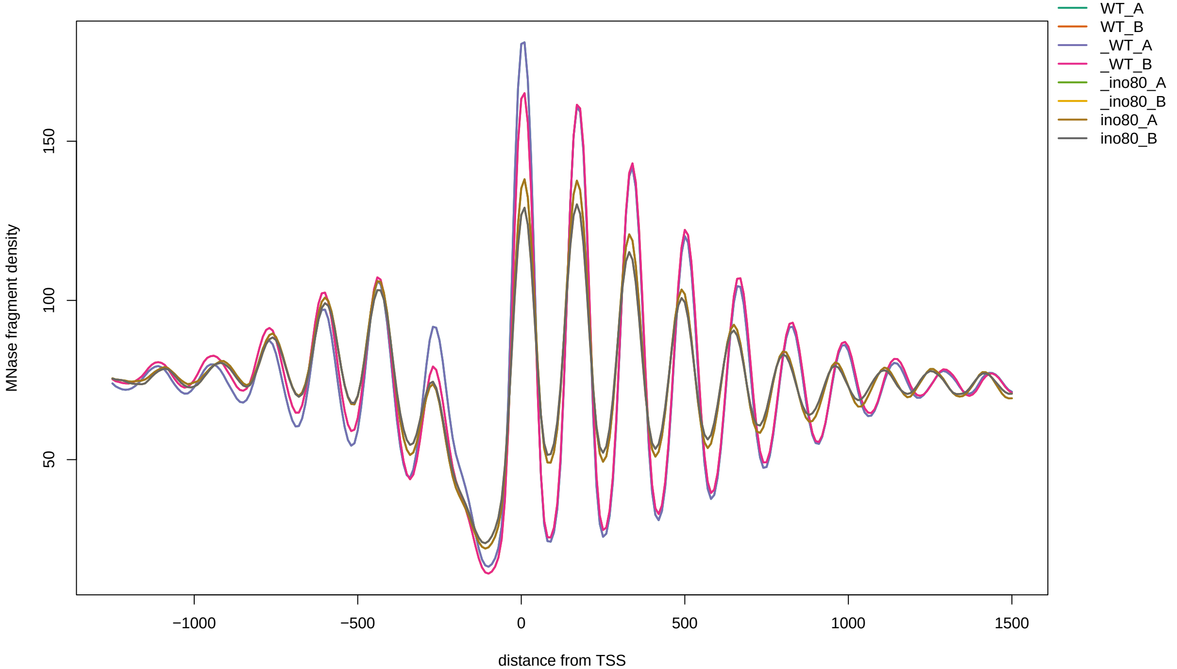
TSS profile: all samples (./plus1_tandem_out_plot/plus1_tandem_out_plot)
