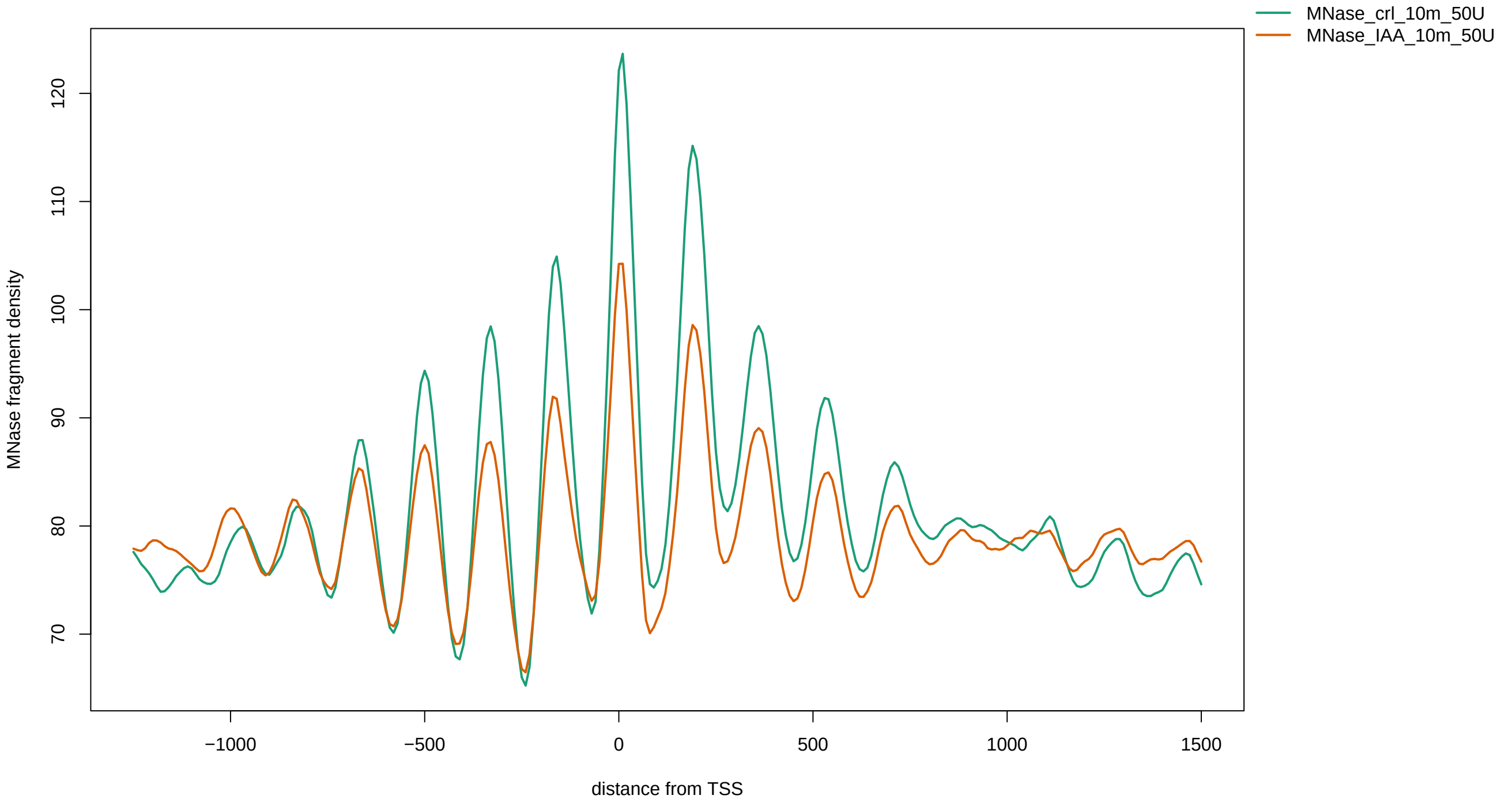
MNase_crl_10m_50U vs MNase_IAA_10m_50U
