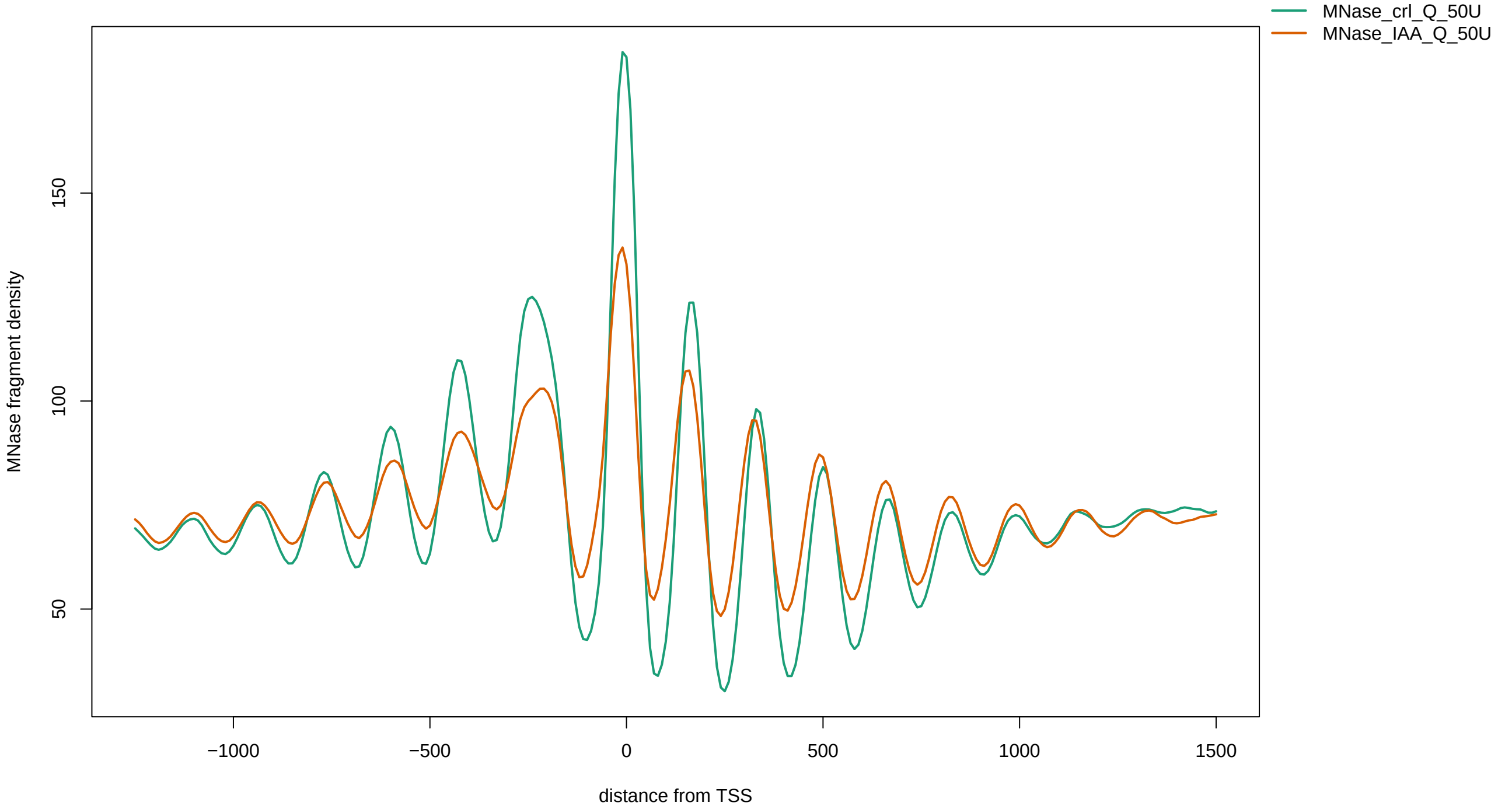
MNase_crl_Q_50U vs MNase_IAA_Q_50U
