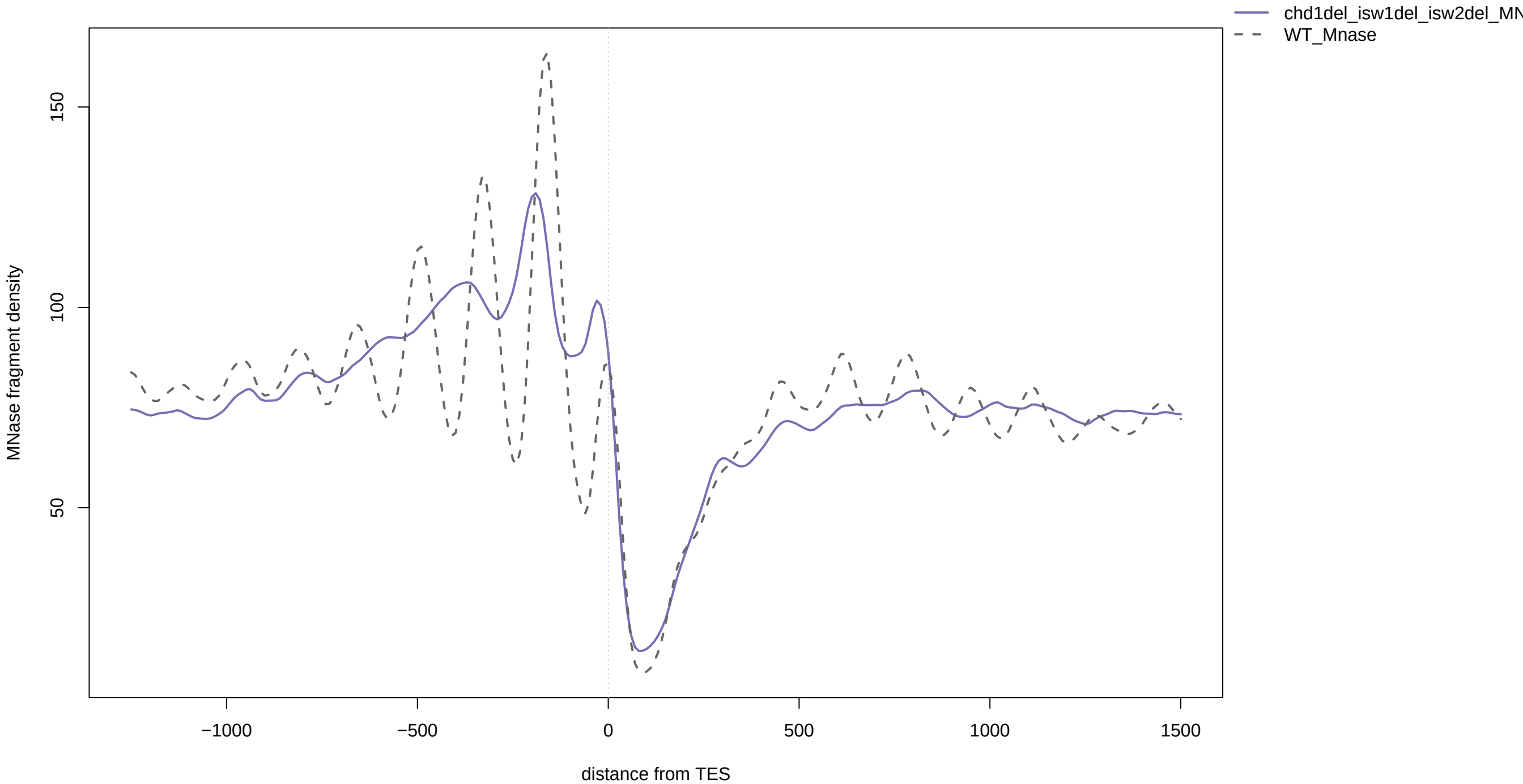
chd1del_isw1del_isw2del_MNase vs WT_Mnase
