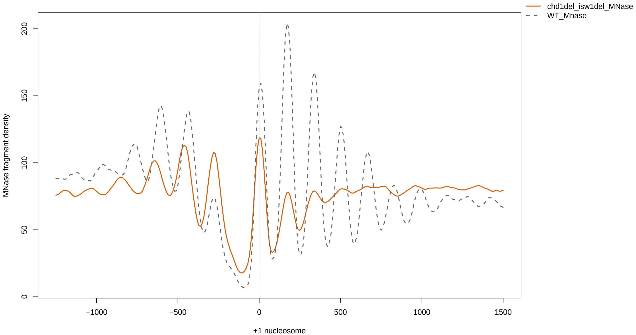
chd1del_isw1del_MNase vs WT_Mnase
