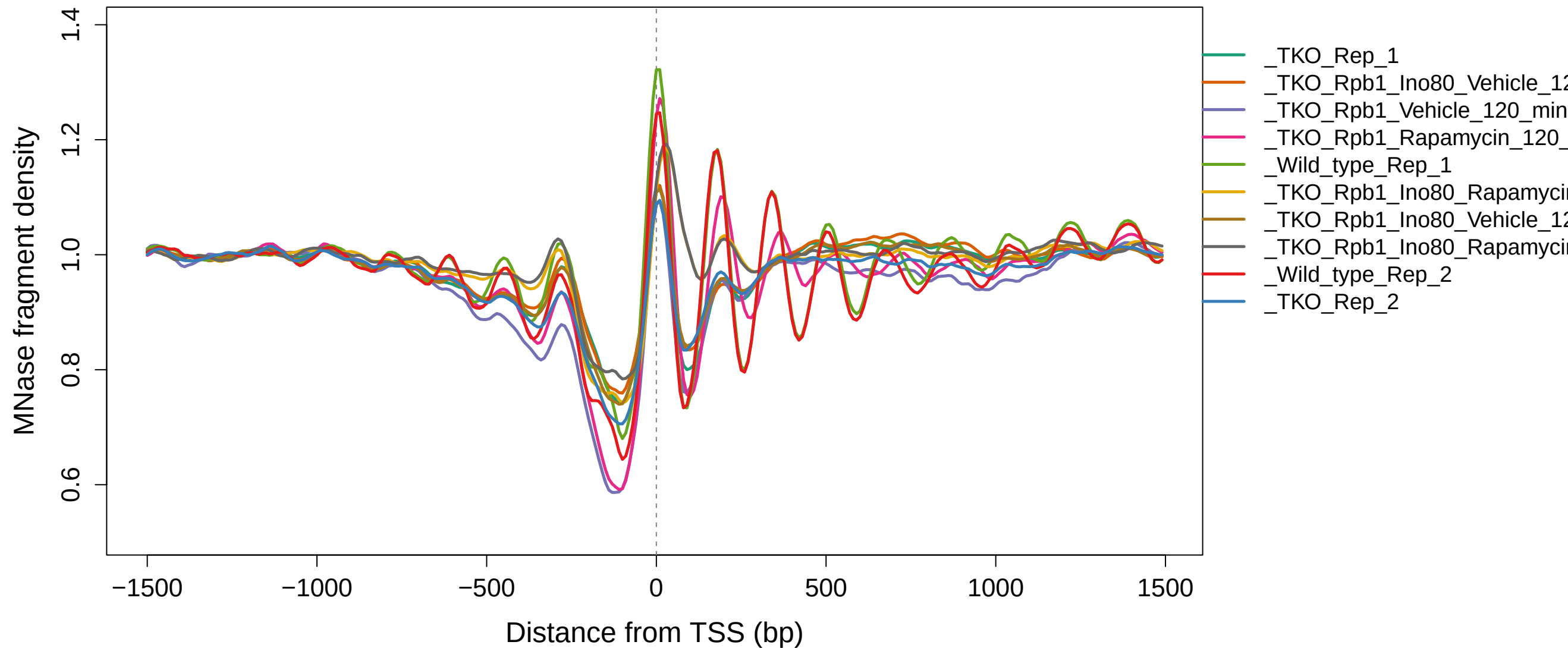
TSS profile – all samples (genes \leq 1000 bp)
