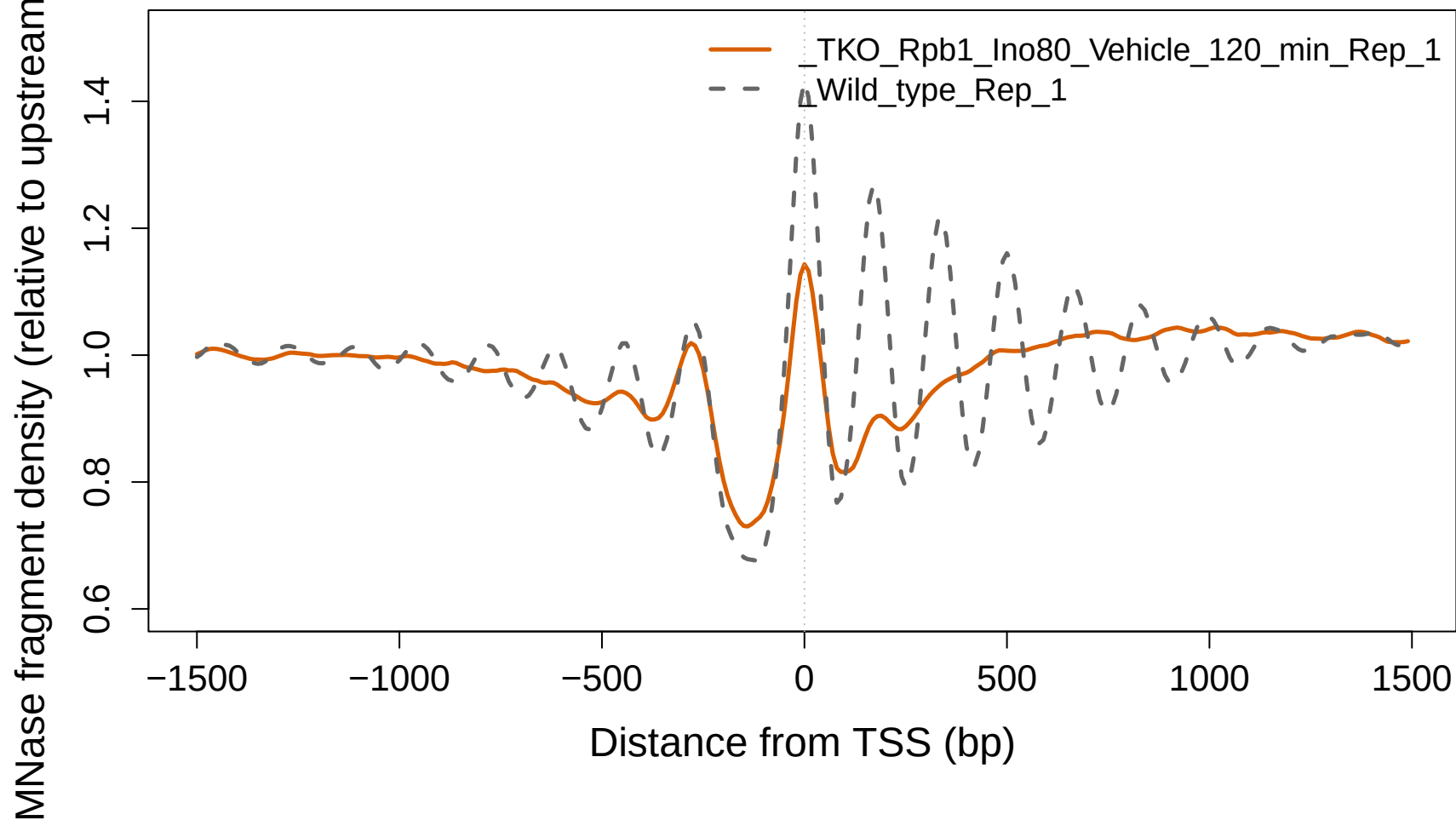
TSS profile - _TKO_Rpb1_Ino80_Vehicle_120_min_Rep_1 vs _Wild_type_Re
