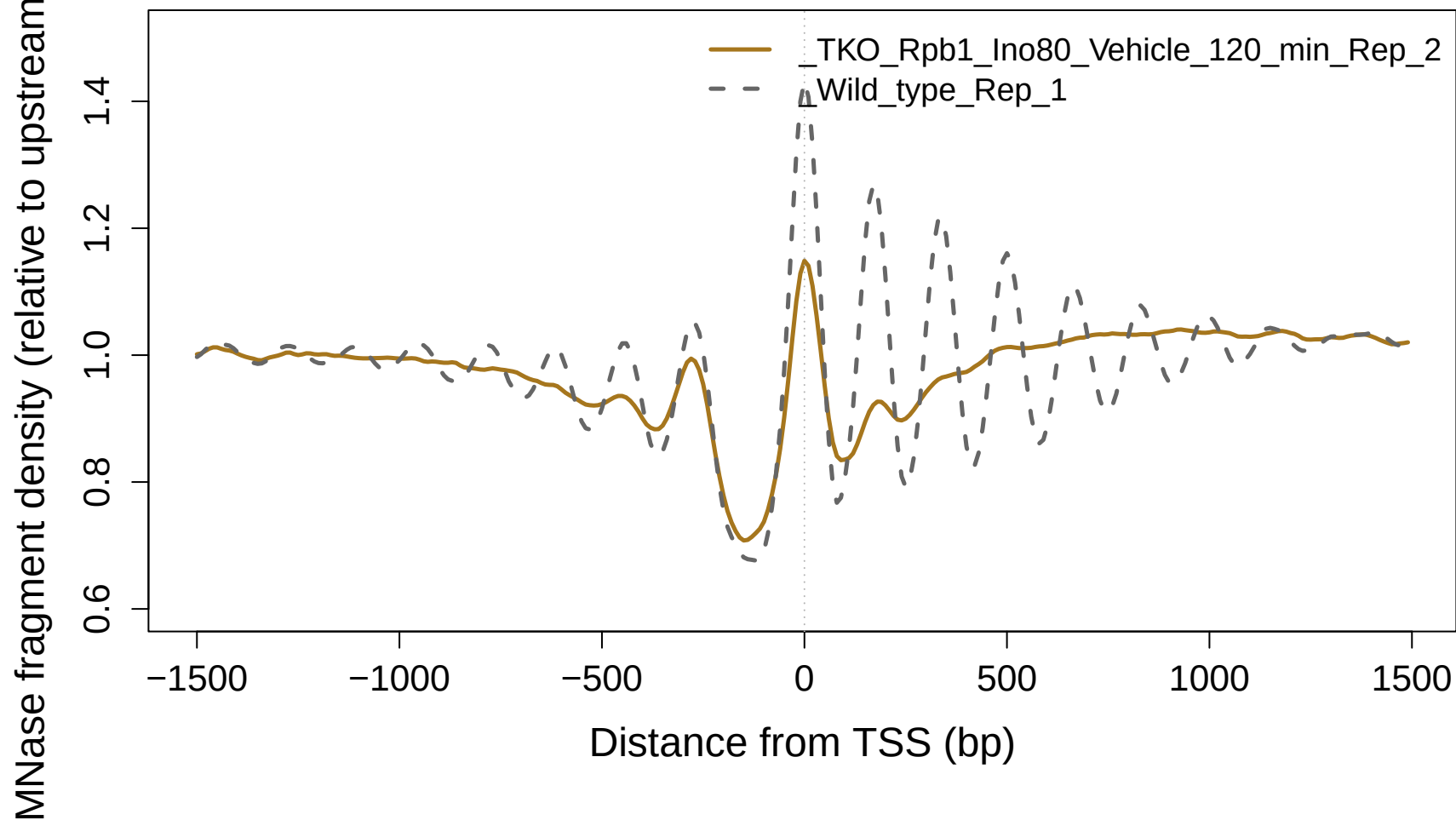
TSS profile - _TKO_Rpb1_Ino80_Vehicle_120_min_Rep_2 vs _Wild_type_Re
