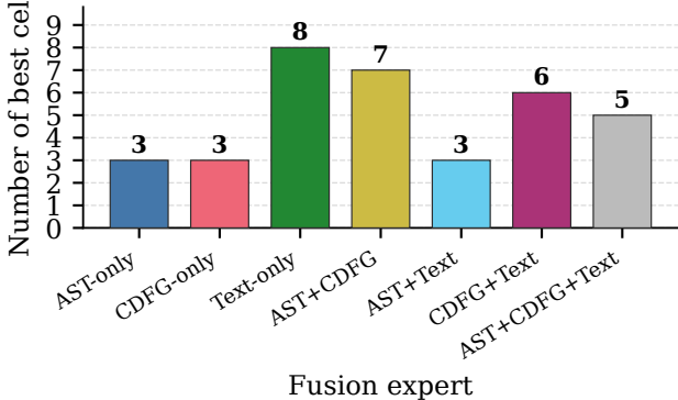
Best fixed expert across 35 (kernel, QoR) pairs
