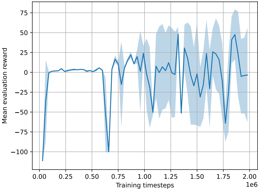
PPO performance on MultiWalker
