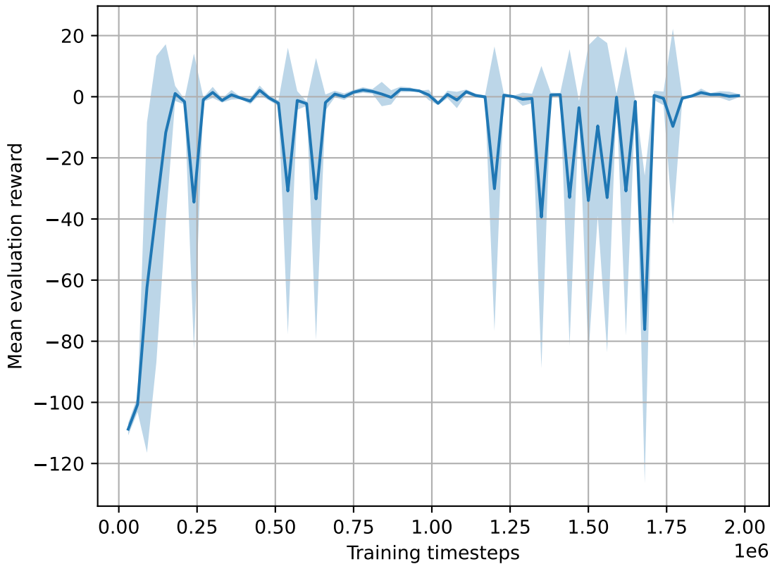
SAC performance on MultiWalker
