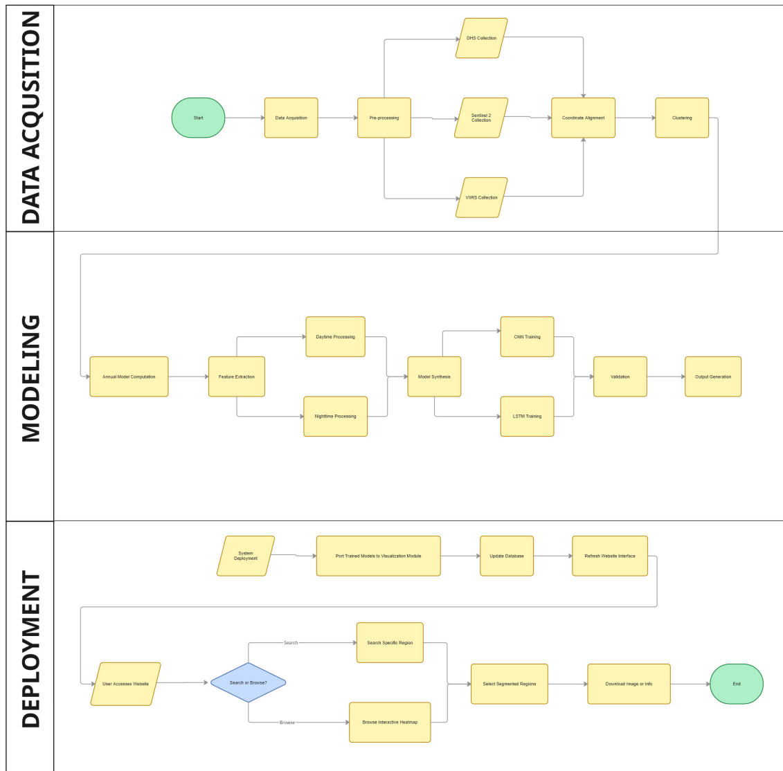
Figure 3: Activity diagram
