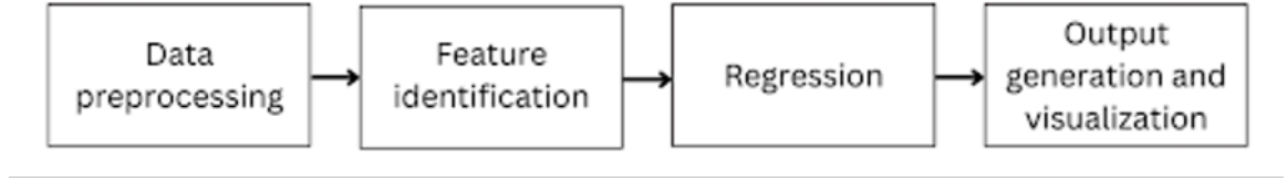
Figure 5: Component diagram
