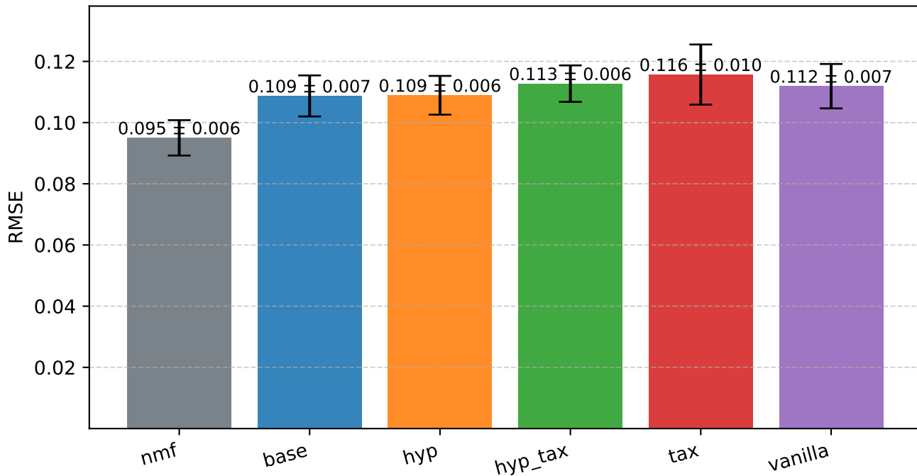
Reconstruction metrics
