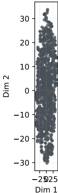
t-SNE (latent)
