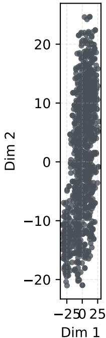
t-SNE (original)
