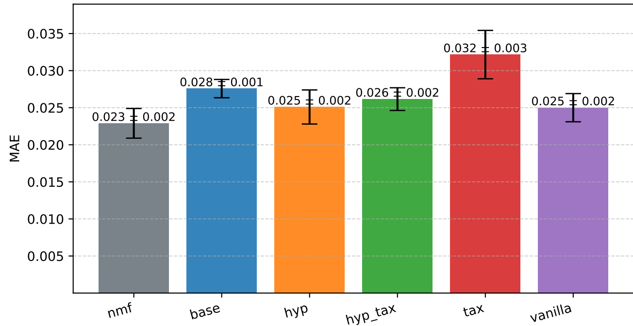
Benchmark Overview
