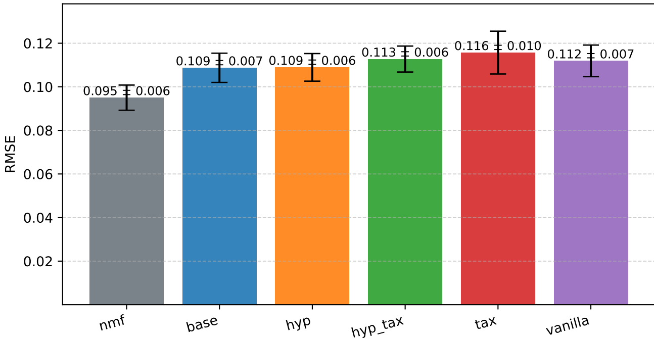
Benchmark Overview
