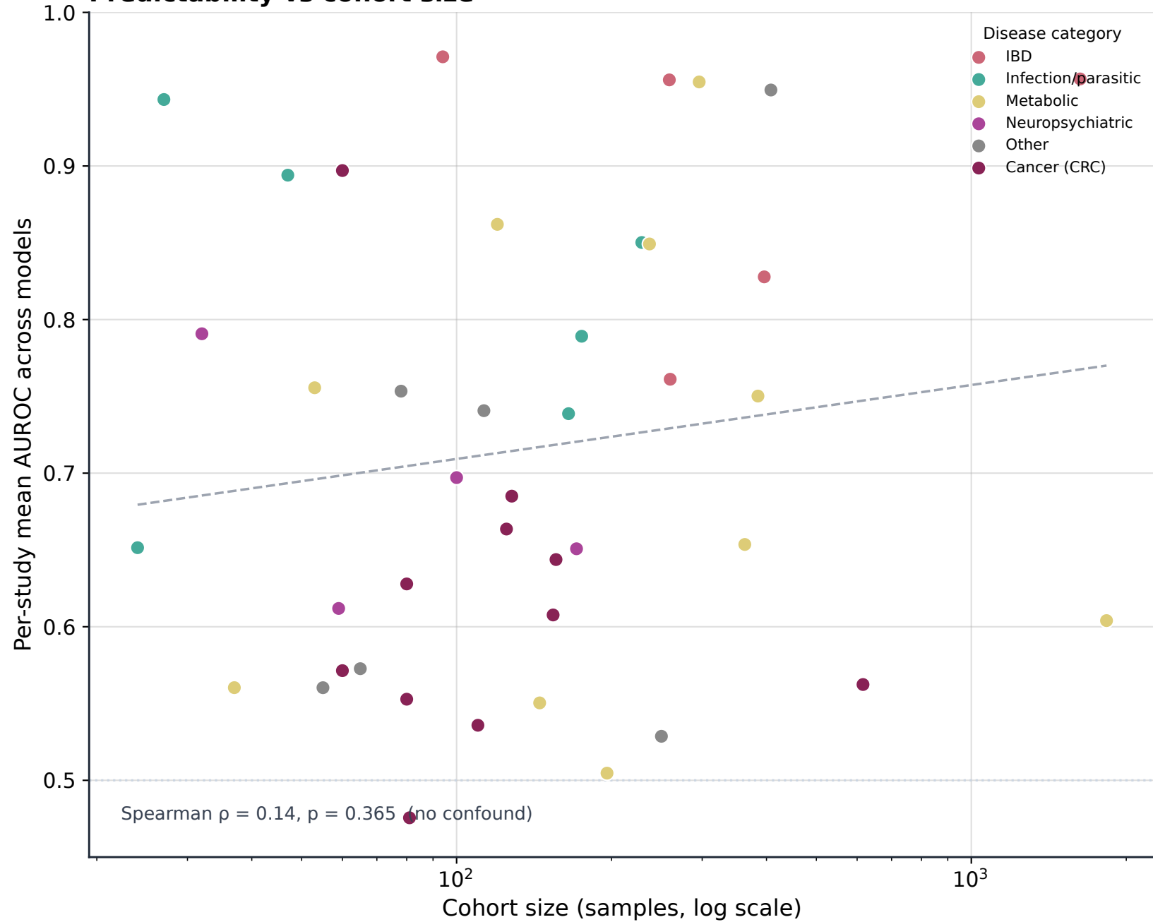
Predictability vs cohort size
