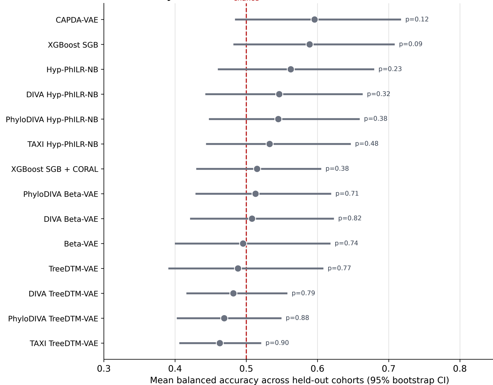
A Does any model beat chance under strict LOSO?
