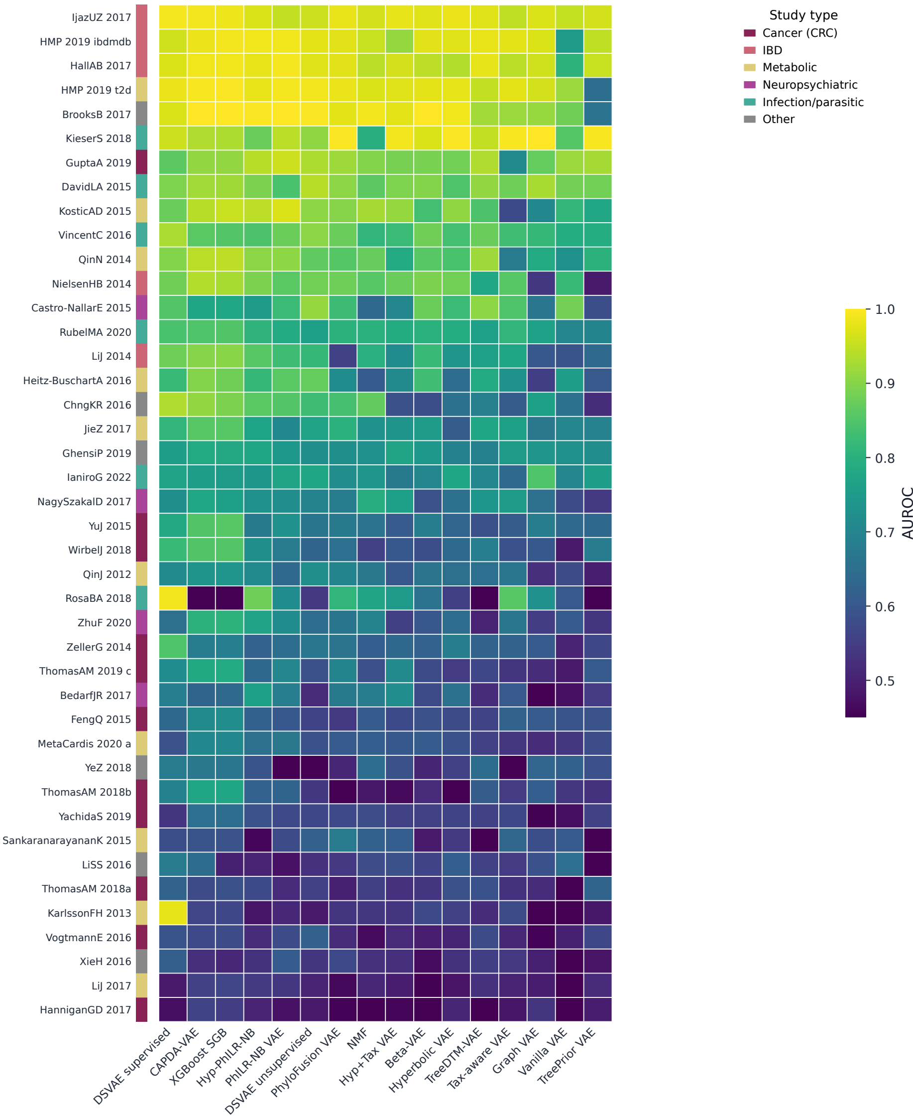
AUROC by study and model
