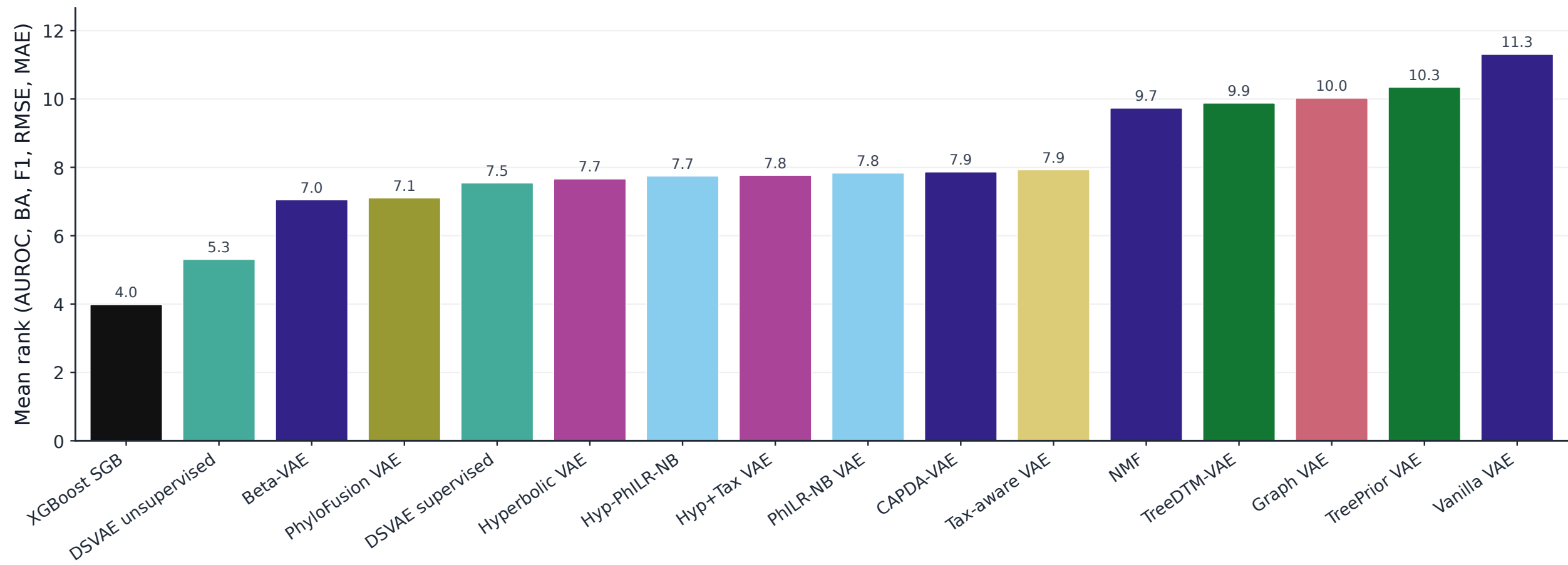
Overall multi-metric ordering (lower rank is better)
