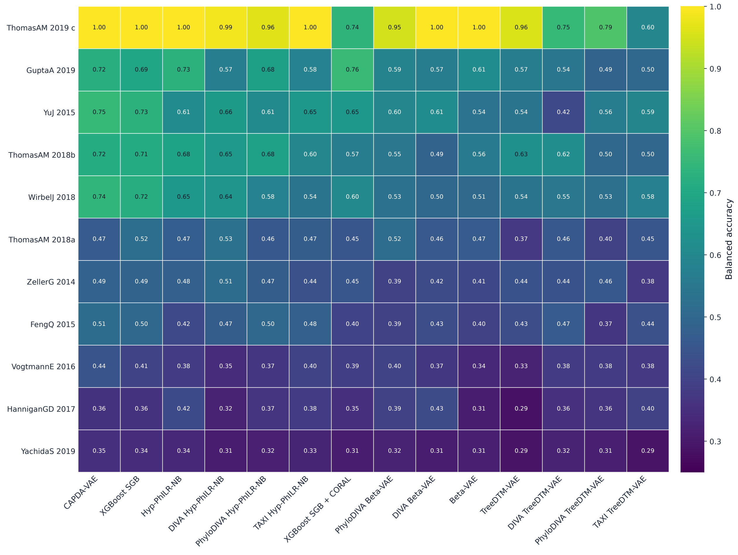
Balanced accuracy by held-out study
