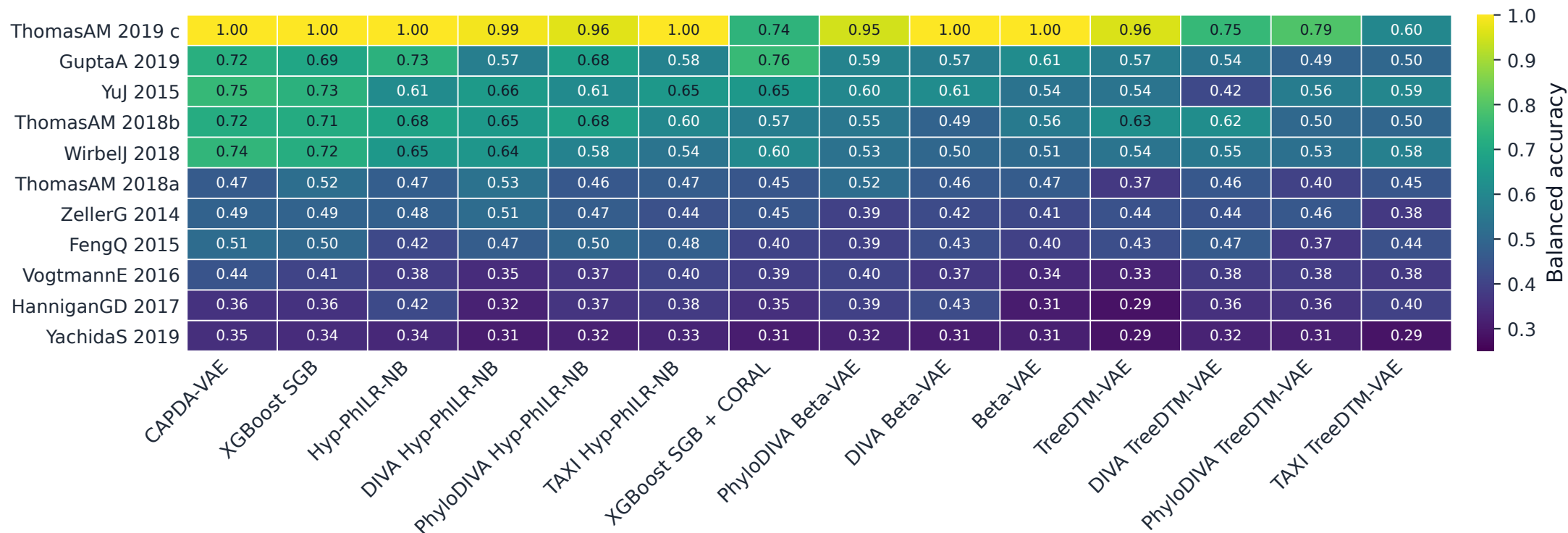
Balanced accuracy by held-out study
