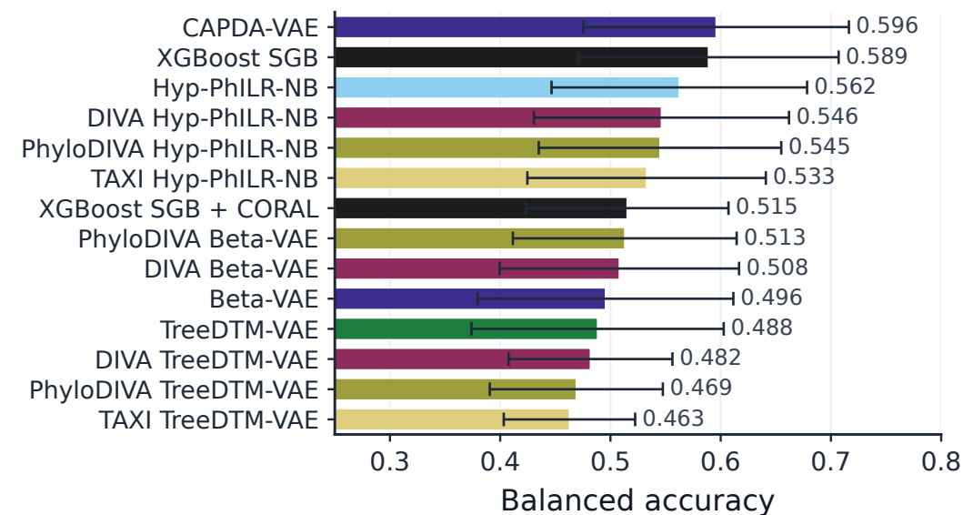
Strict LOSO balanced accuracy
