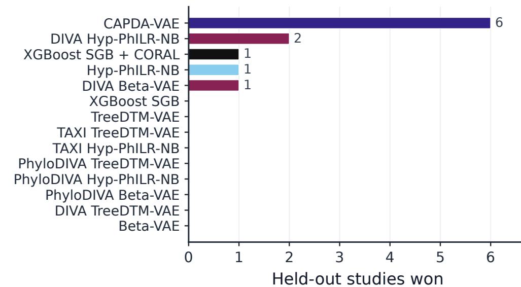
Best-model frequency
