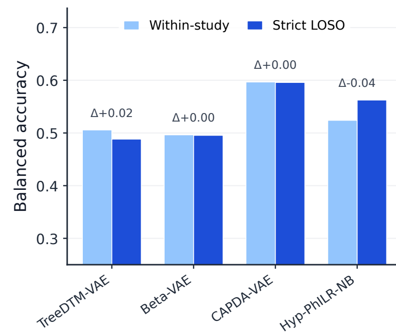
Within-study → LOSO transfer gap
