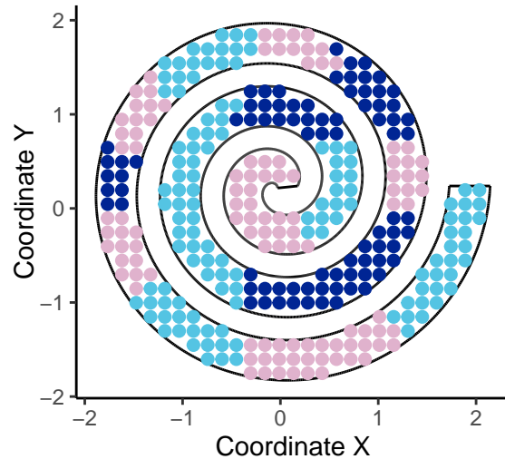
k = 20, c = 3, ARI = 0.801
