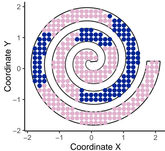
k = 8, c = 2, ARI = 0.385
