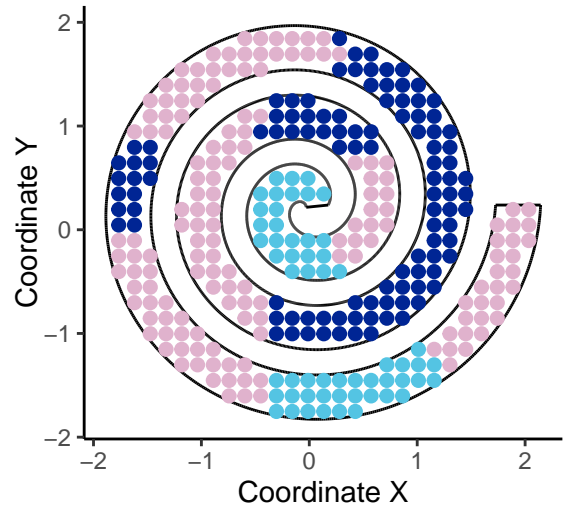
k = 12, c = 3, ARI = 0.504
