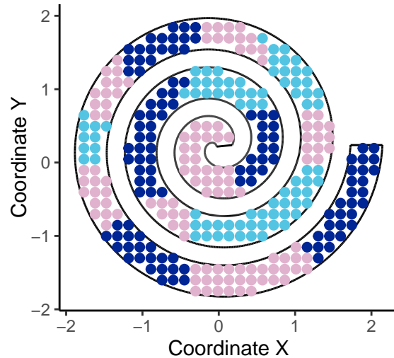
k = 24, c = 3, ARI = 0.836
