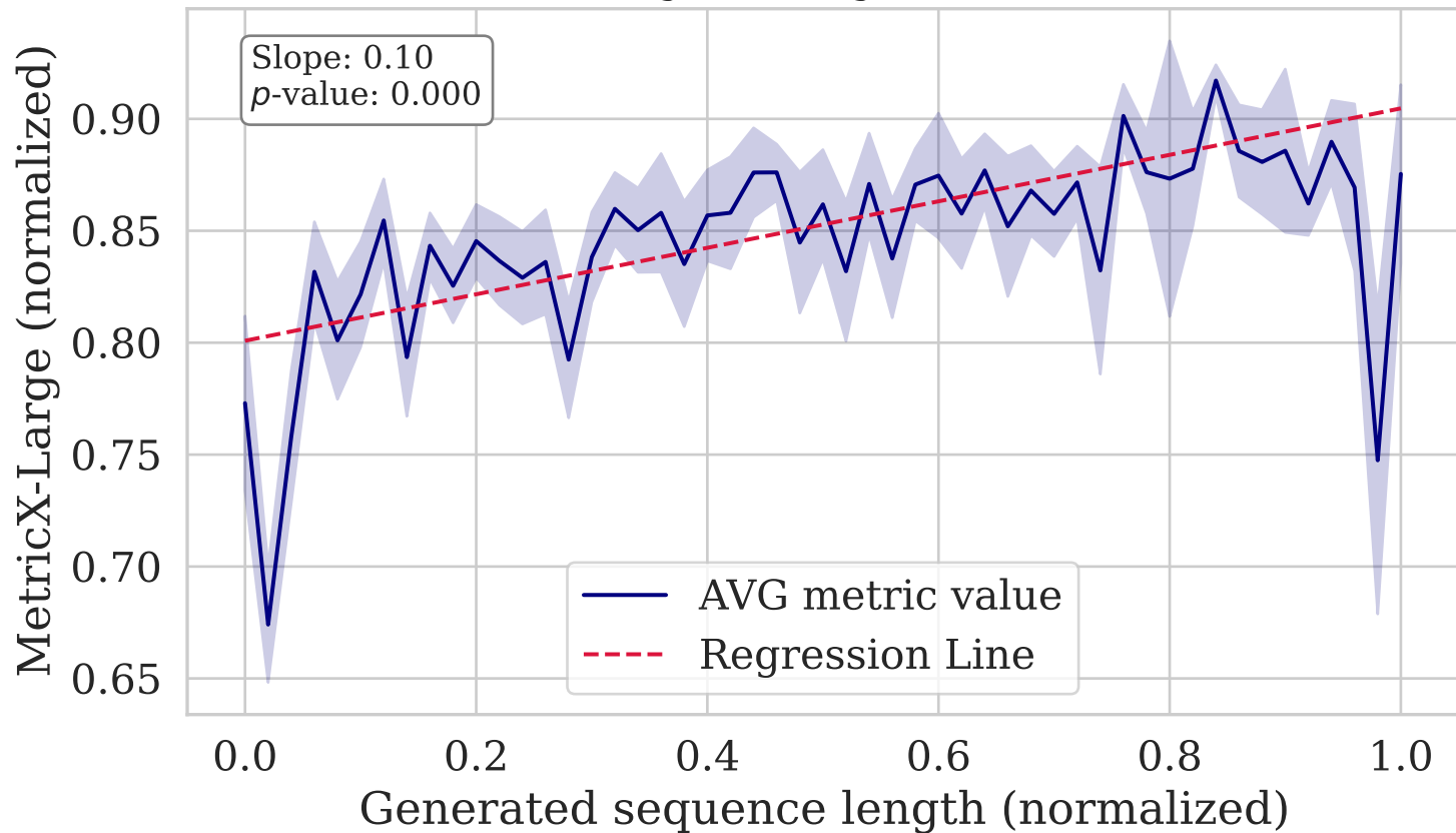
MetricX-Large vs. Length (WMT19 Fi-En)
