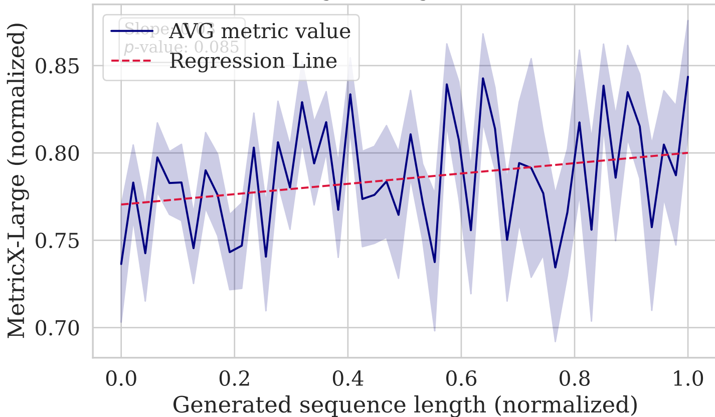
MetricX-Large vs. Length (WMT19 Lt-En)
