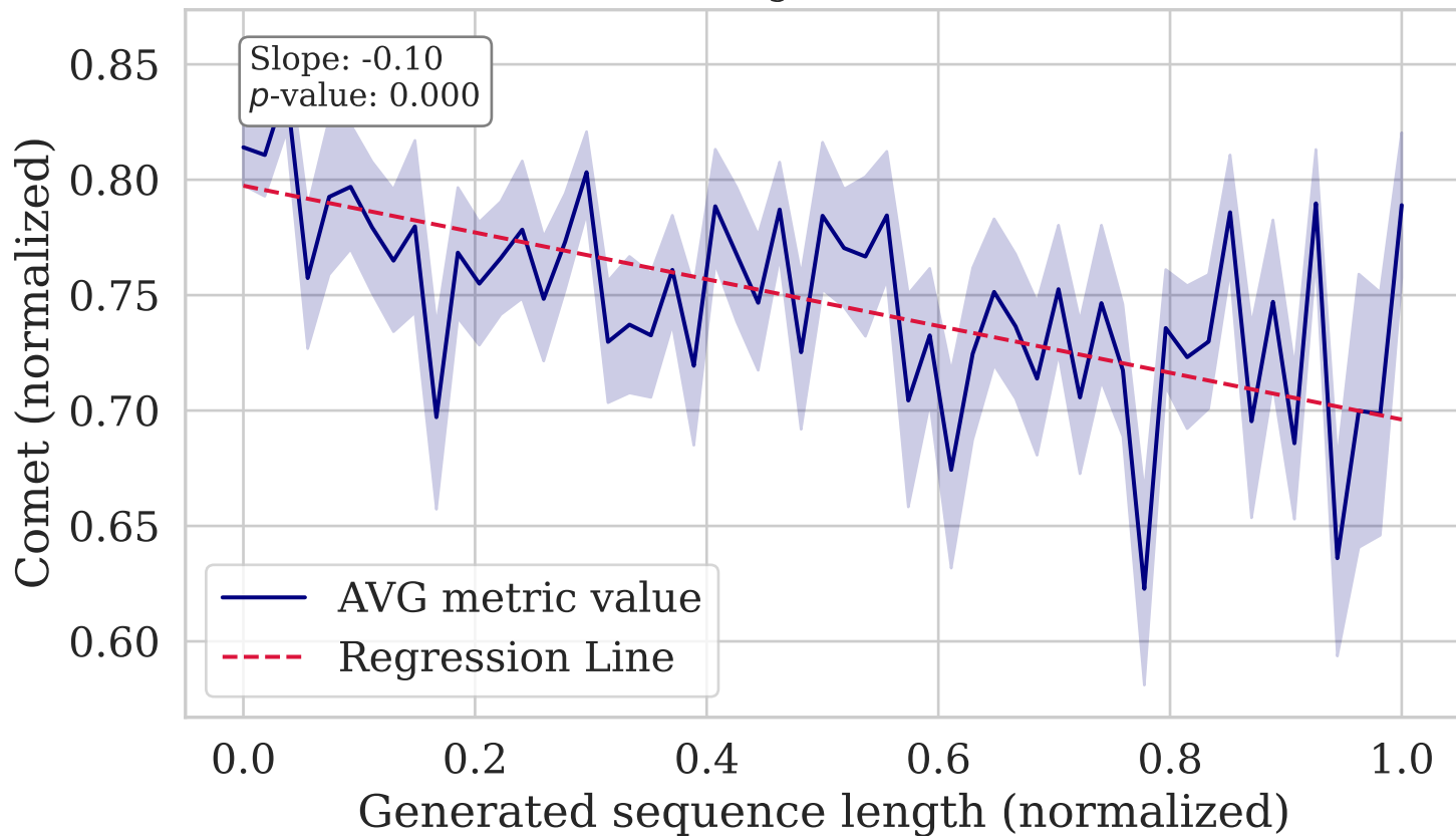
Comet vs. Length (WMT14 Ru-En)
