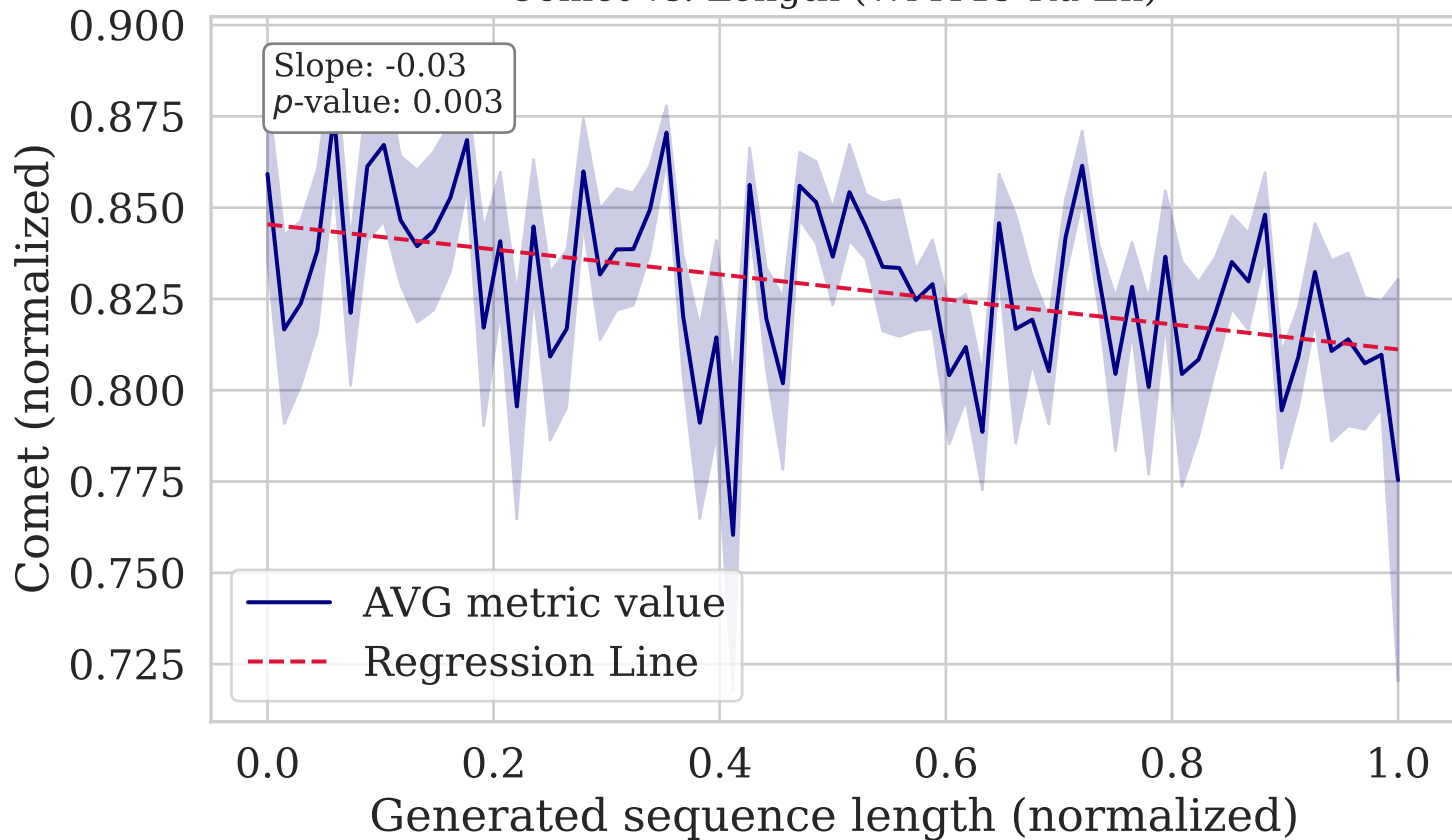
Comet vs. Length (WMT19 Ru-En)
