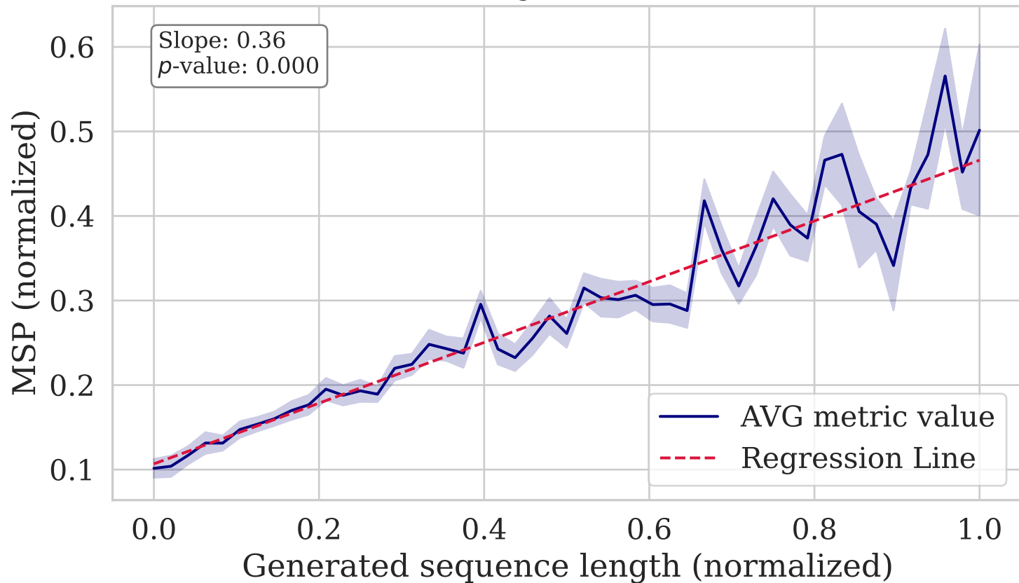
MSP vs. Length (WMT14 De-En)
