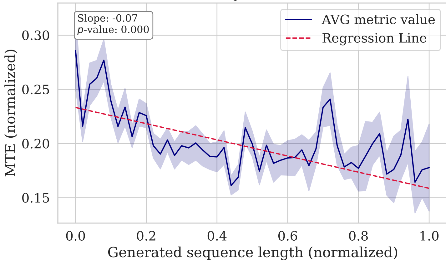
MTE vs. Length (WMT19 Fi-En)
