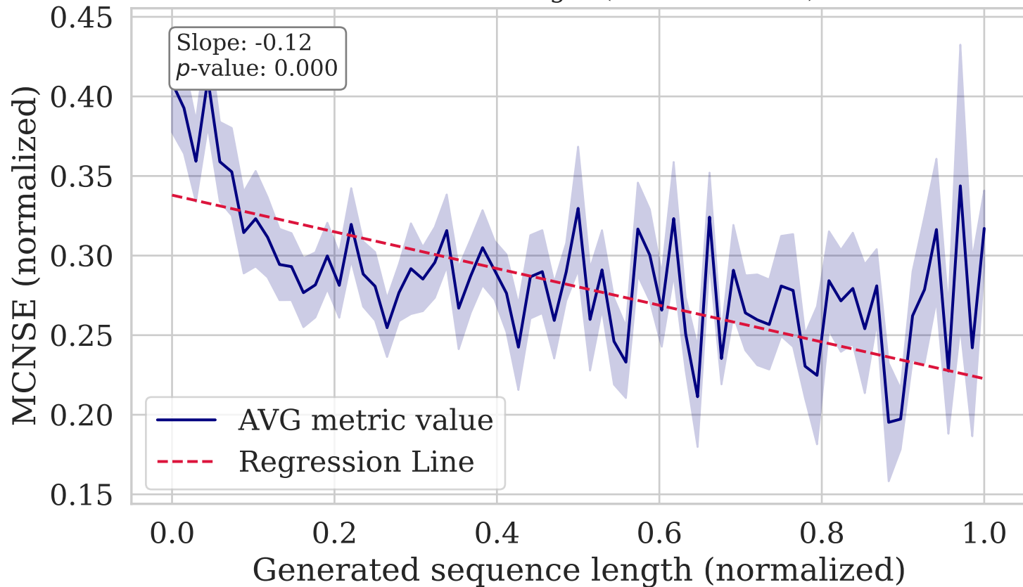
MCNSE vs. Length (WMT19 Ru-En)
