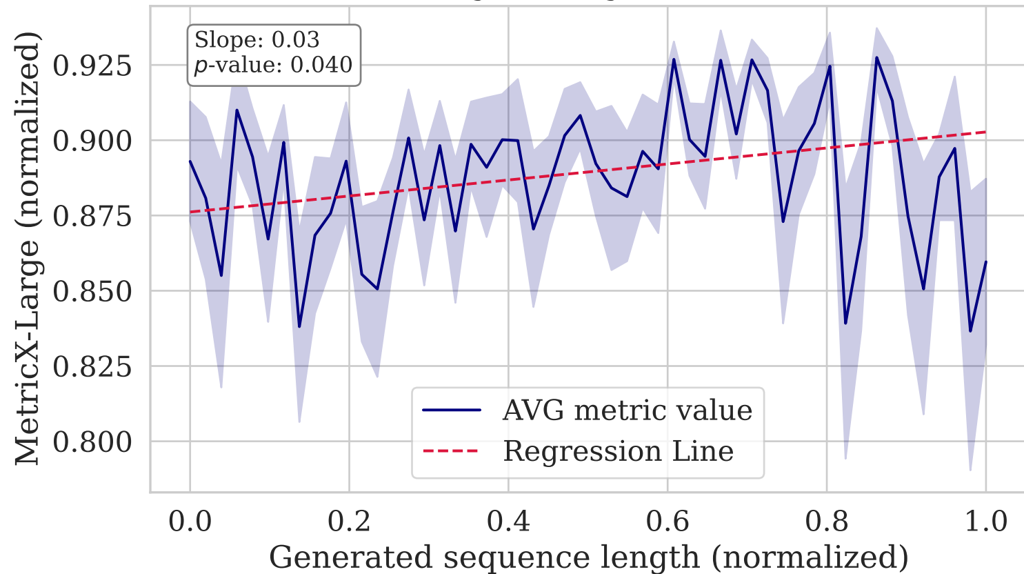
MetricX-Large vs. Length (WMT14 Cs-En)
