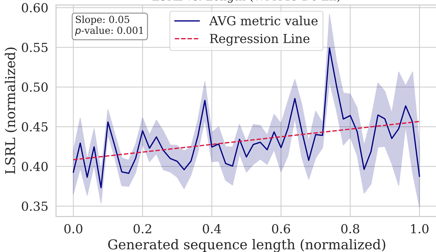
LSRL vs. Length (WMT19 De-En)
