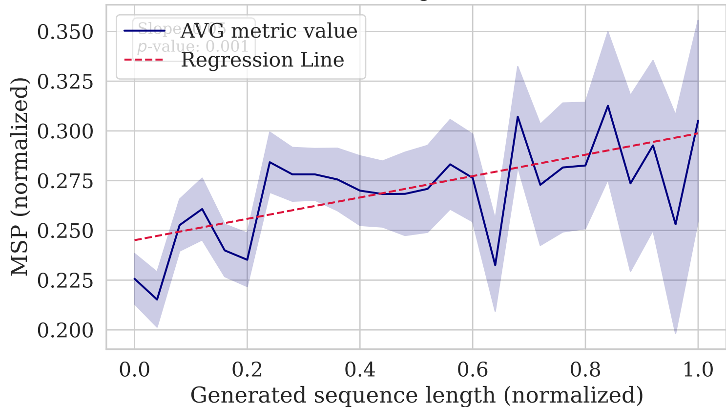
MSP vs. Length (XSUM)
