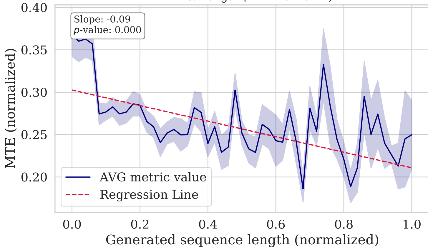
MTE vs. Length (WMT19 De-En)
