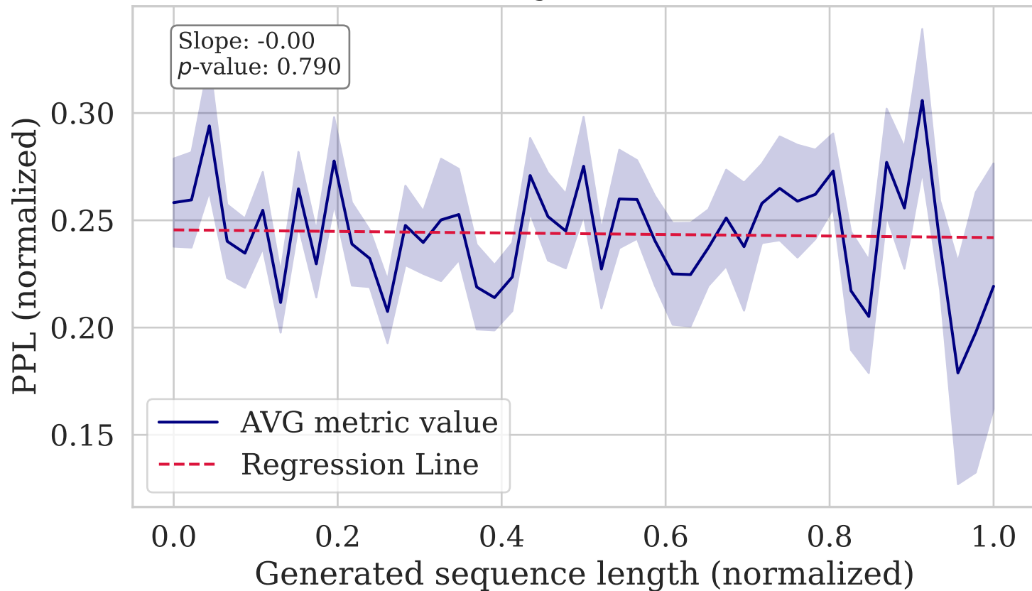
PPL vs. Length (WMT19 Fi-En)
