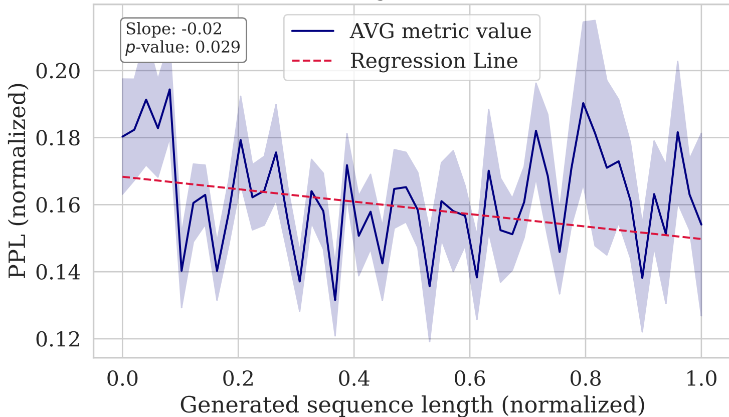
PPL vs. Length (WMT19 Lt-En)
