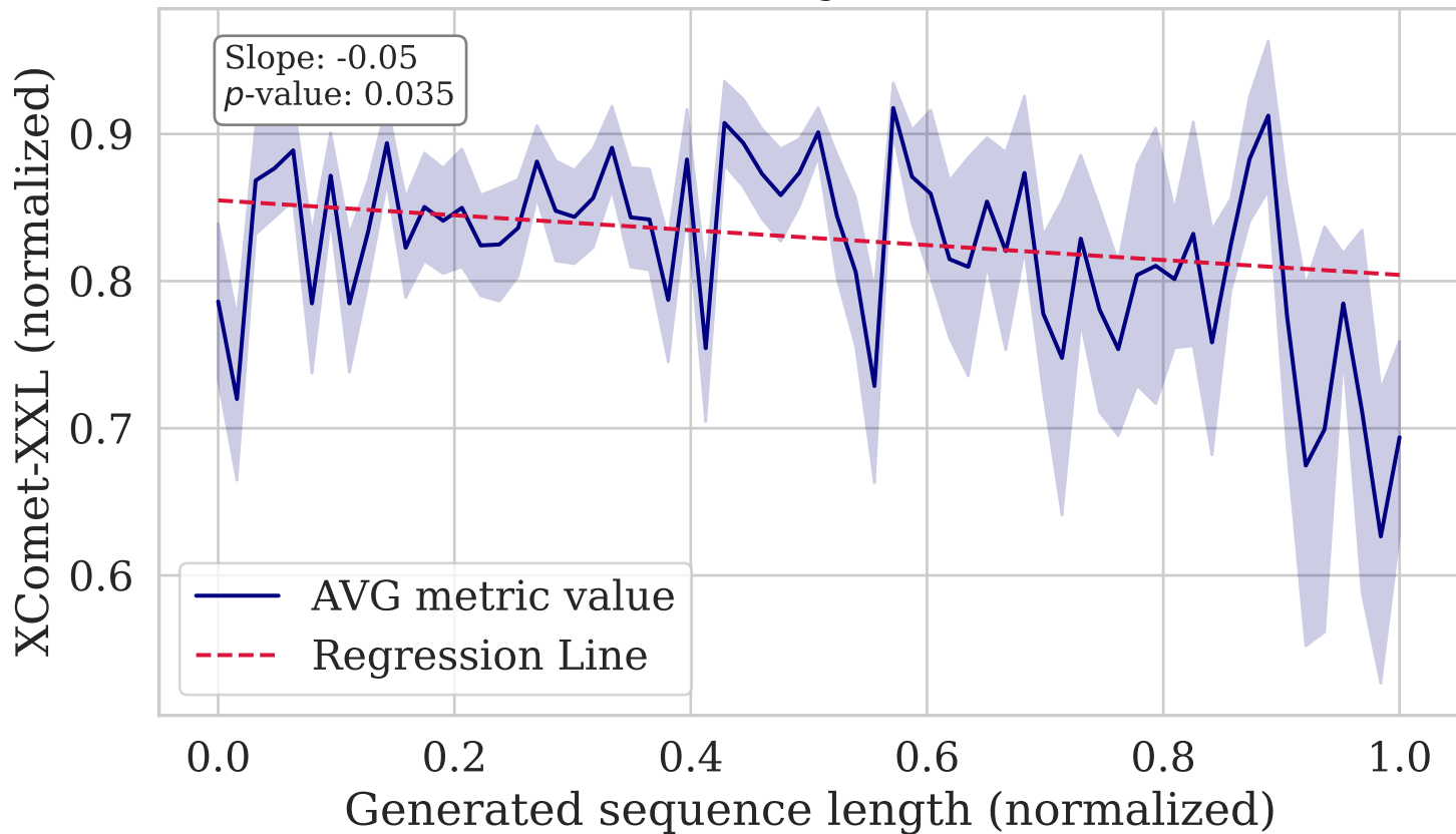
XComet-XXL vs. Length (WMT14 Fr-En)
