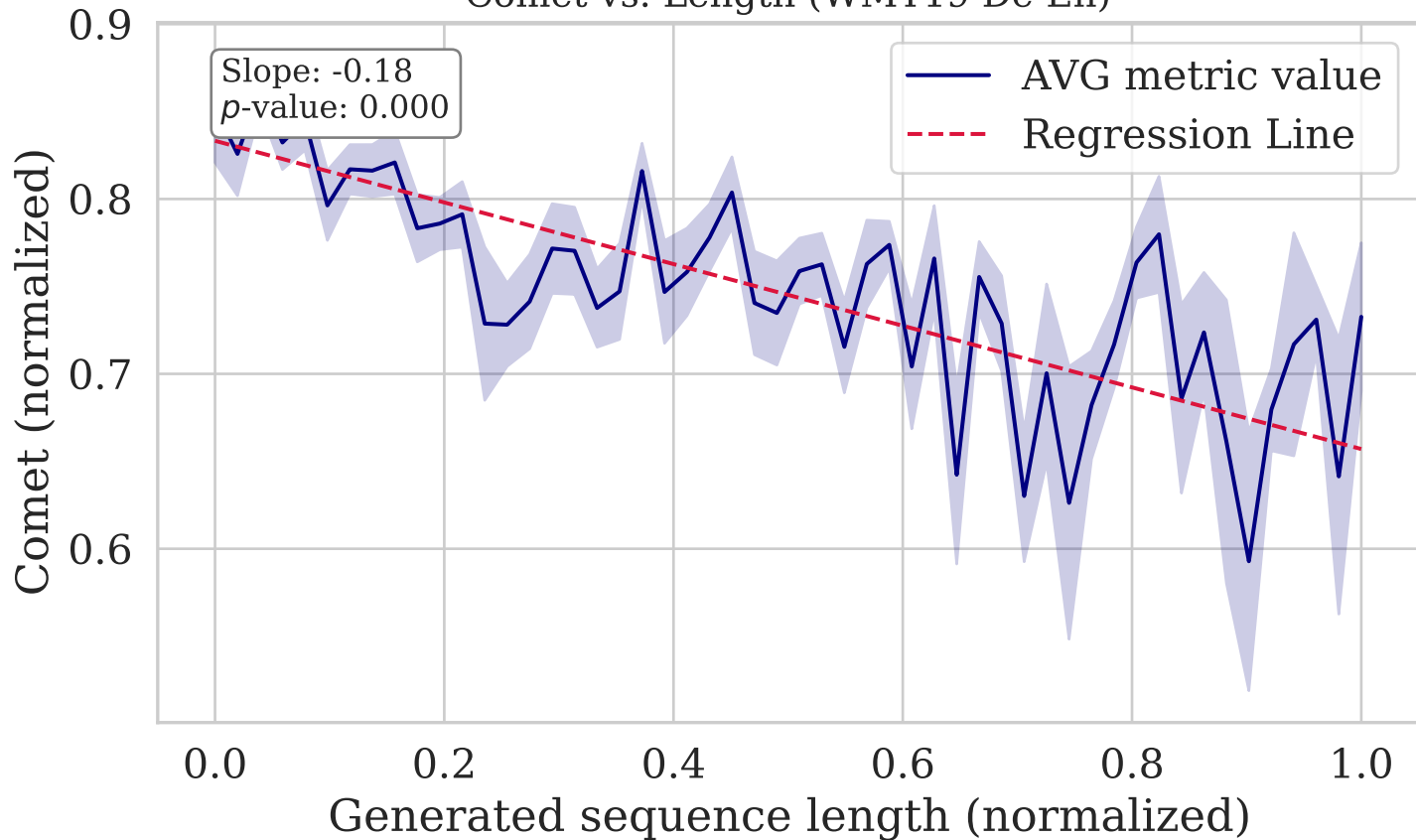
Comet vs. Length (WMT19 De-En)
