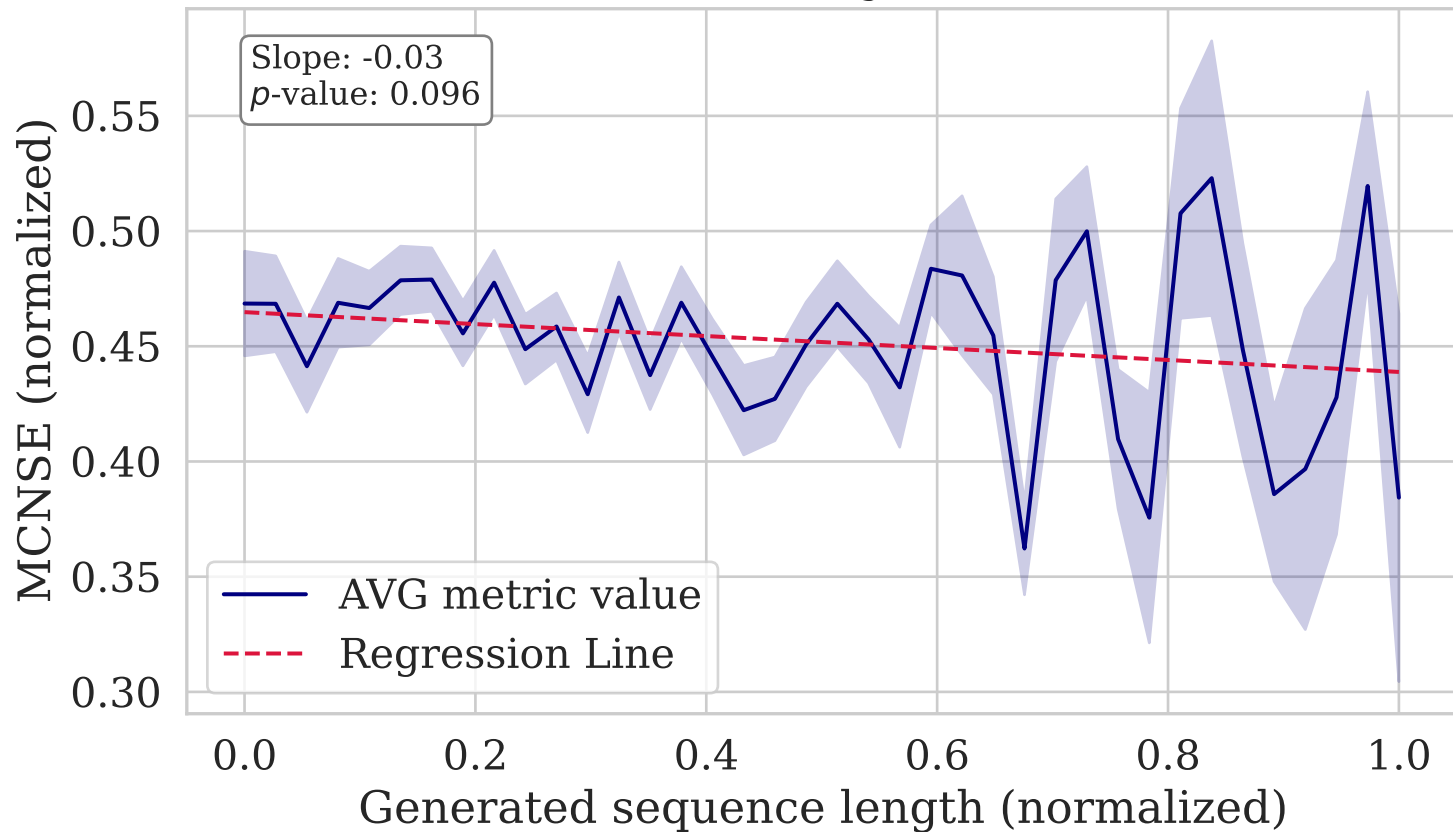
MCNSE vs. Length (XSUM)
