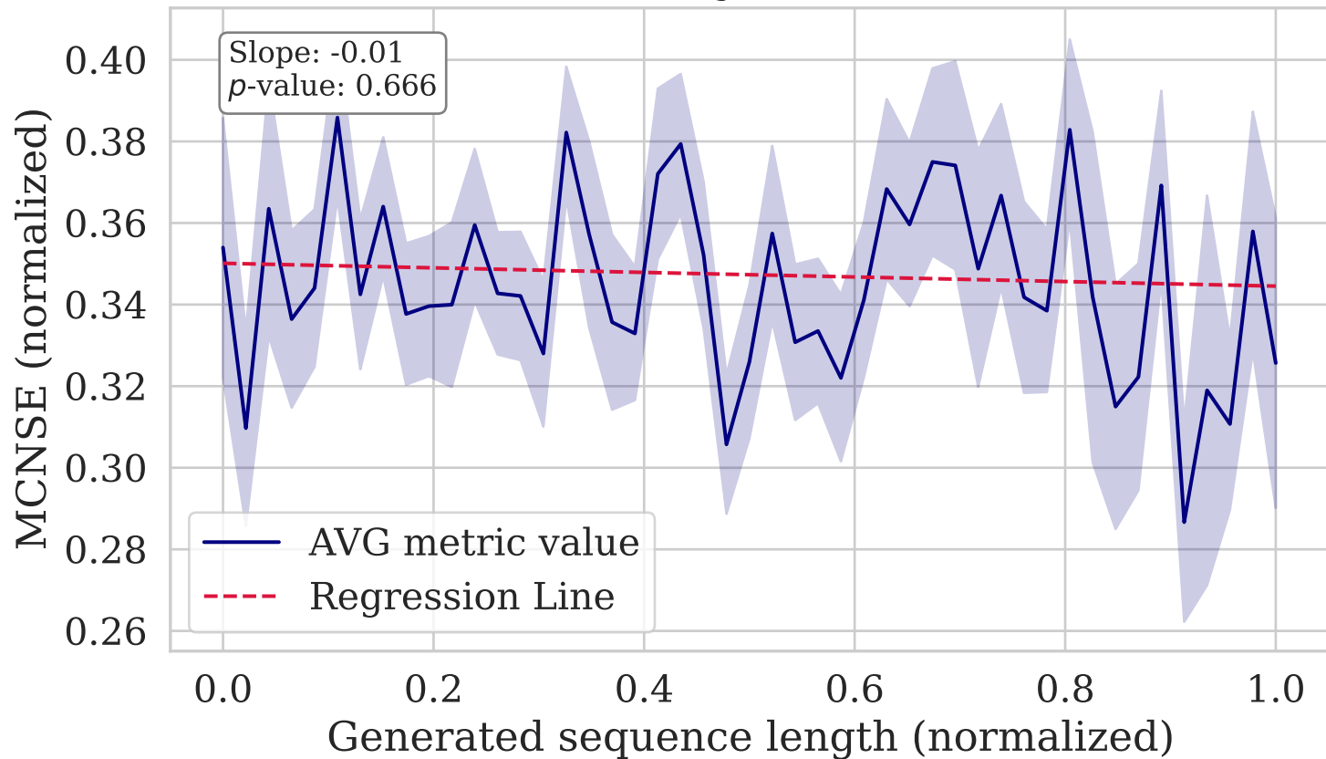
MCNSE vs. Length (WMT14 De-En)
